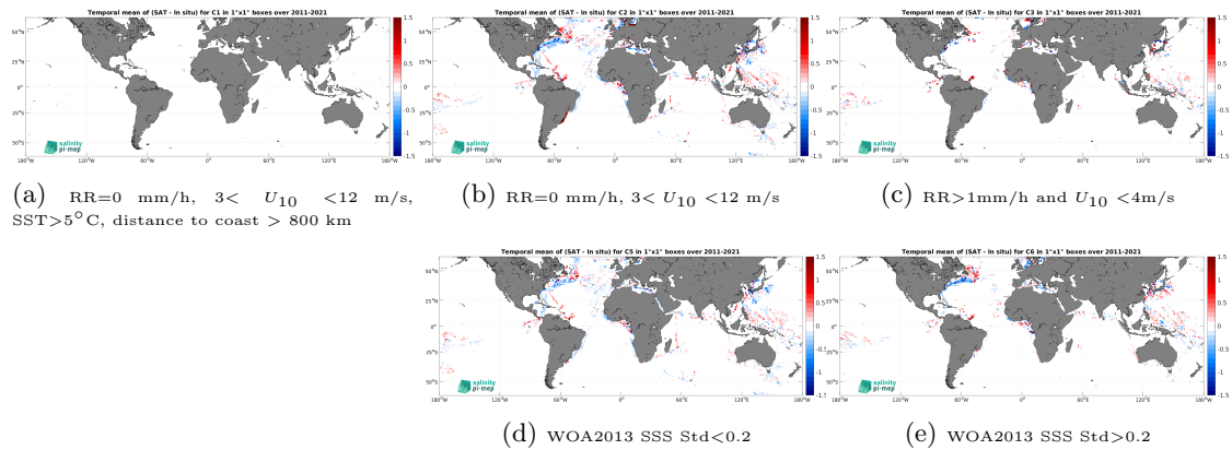
Figure 12: Temporal mean gridded over spatial boxes of size 1^\circ \times 1^\circ of \Delta\text{SSS} (SMOS SSS L4 v2 - Daily (BEC) - TSG (LEGOS-DM)) for 5 different subdatasets corresponding to:RR=0 mm/h, 3 < U_{10} < 12 m/s, SST >5^\circ\text{C} , distance to coast > 800 km (a), RR=0 mm/h, 3 < U_{10} < 12 m/s (b), RR >1 mm/h and U_{10} < 4 m/s (c), WOA2013 SSS Std <0.2 (d), WOA2013 SSS Std >0.2 (e).
