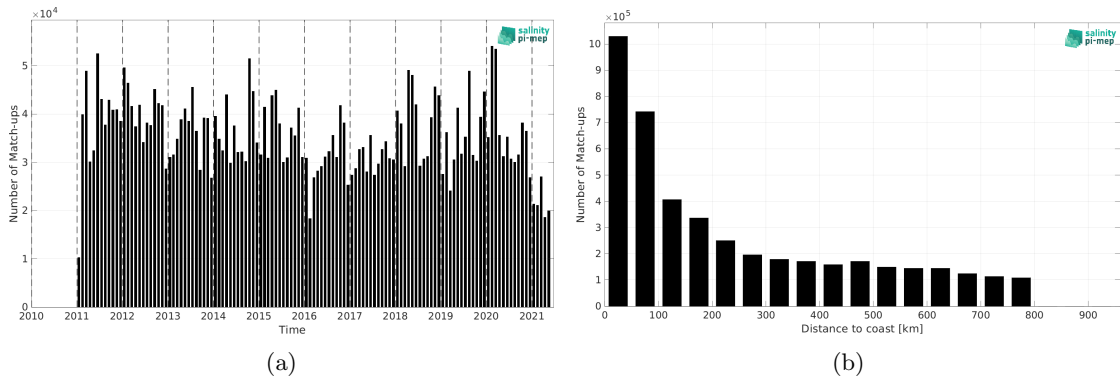
Figure 1: Number of match-ups between TSG (LEGOS-DM) and SMOS SSS L4 v2 - Daily (BEC) SSS as a function of time (a) and as function of the distance to coast (b) over the SMOS coastal zone (<800km) 60N-60S Pi-MEP region and for the full satellite product period.
