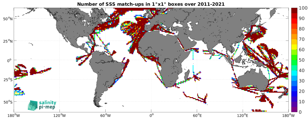
Figure 4: Number of SSS match-ups between TSG (LEGOS-DM) SSS and the SMOS SSS L4 v2 - Daily (BEC) SSS product for the SMOS coastal zone (<800km) 60N-60S Pi-MEP region over 1^\circ \times 1^\circ boxes and for the full satellite product period.
