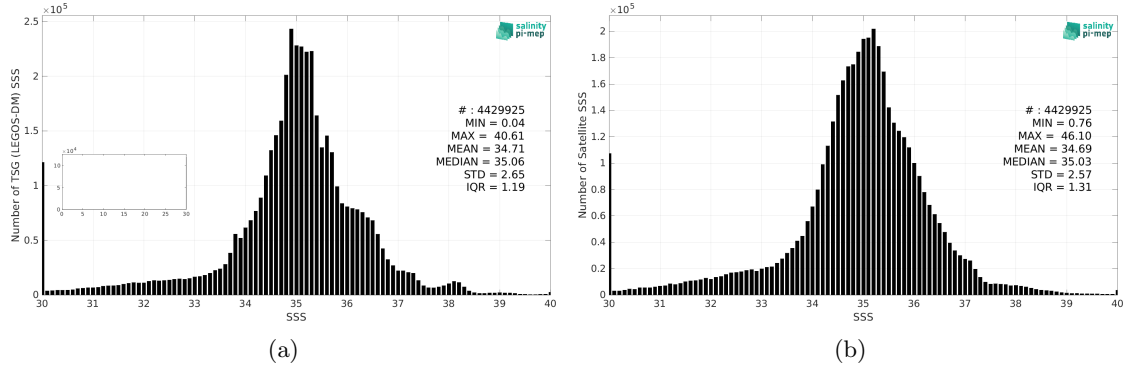
Figure 2: Histograms of SSS from TSG (LEGOS-DM) (a) and SMOS SSS L4 v2 - Daily (BEC) (b) considering all match-up pairs per bins of 0.1 over the SMOS coastal zone (<800km) 60N-60S Pi-MEP region and for the full satellite product period.
