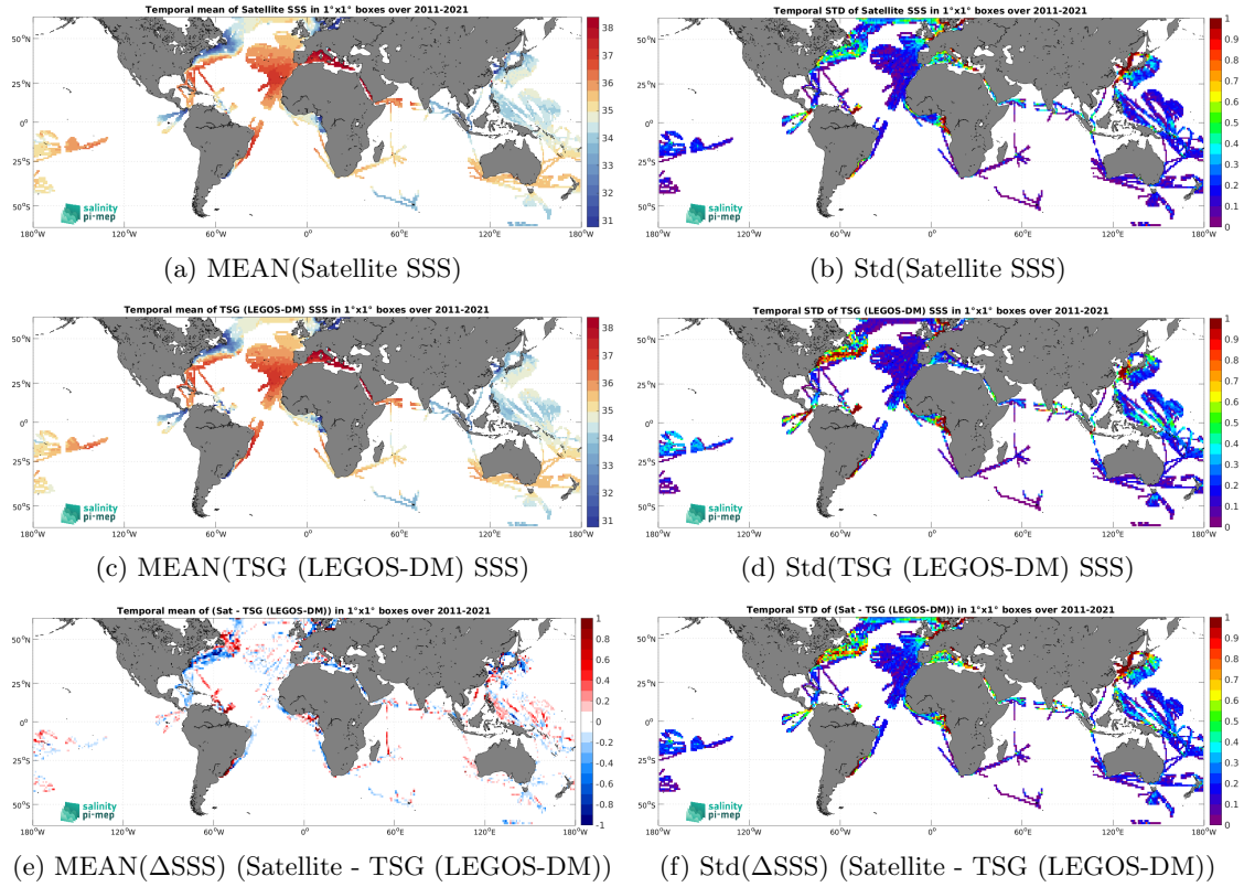
Figure 6: Temporal mean (left) and Std (right) of SSS from SMOS SSS L4 v2 - Daily (BEC) (top), TSG (LEGOS-DM) (middle), and of \Delta SSS (Satellite - TSG (LEGOS-DM)). Only match-up pairs are used to generate these maps.
