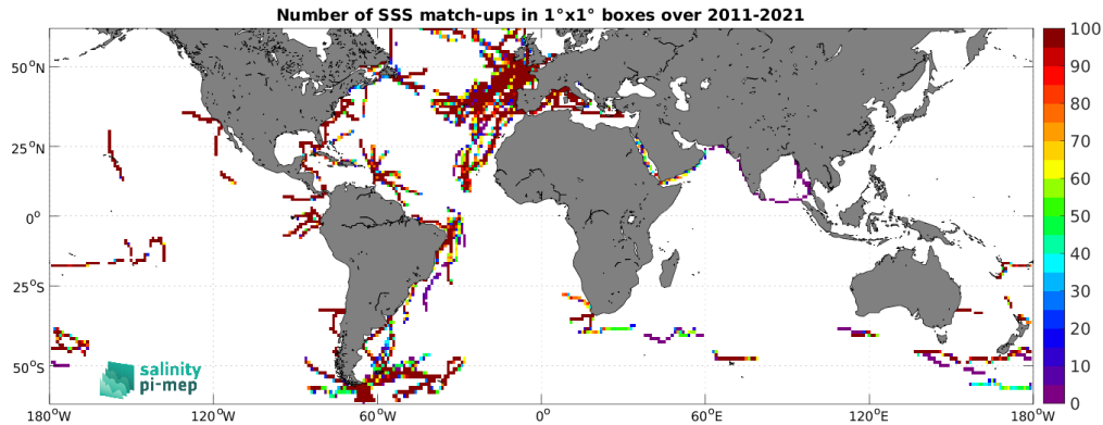
Figure 5: Number of SSS match-ups between TSG (GOSUD-Sailing-ship) SSS and the SMOS SSS L4 v2 - Daily (BEC) SSS product for the SMOS coastal zone (<800km) 60N-60S Pi-MEP region over 1^{\circ} \times 1^{\circ} boxes and for the full satellite product period.
