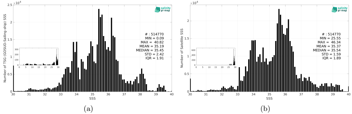
Figure 3: Histograms of SSS from TSG (GOSUD-Sailing-ship) (a) and SMOS SSS L4 v2 - Daily (BEC) (b) considering all match-up pairs per bins of 0.1 over the SMOS coastal zone (<800km) 60N-60S Pi-MEP region and for the full satellite product period.
