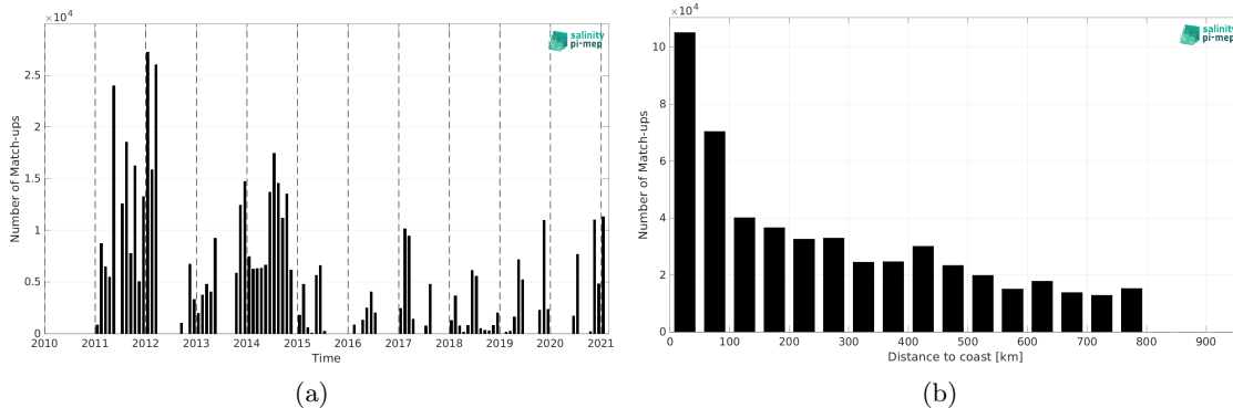
Figure 2: Number of match-ups between TSG (GOSUD-Sailing-ship) and SMOS SSS L4 v2 - Daily (BEC) SSS as a function of time (a) and as function of the distance to coast (b) over the SMOS coastal zone (<800km) 60N-60S Pi-MEP region and for the full satellite product period.
