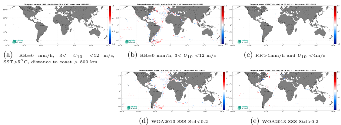
Figure 14: Temporal mean gridded over spatial boxes of size 1^\circ \times 1^\circ of \Delta\text{SSS} (SMOS SSS L4 v2 - Daily (BEC) - TSG (GOSUD-Sailing-ship)) for 5 different subdatasets corresponding to:RR=0 mm/h, 3 < U_{10} < 12 m/s, SST >5^\circ\text{C} , distance to coast > 800 km (a), RR=0 mm/h, 3 < U_{10} < 12 m/s (b), RR >1 mm/h and U_{10} < 4 m/s (c), WOA2013 SSS Std <0.2 (d), WOA2013 SSS Std >0.2 (e).
