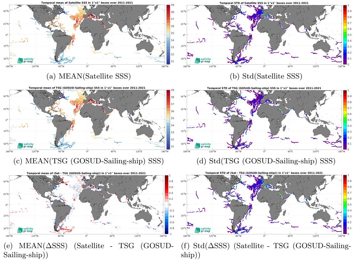
Figure 7: Temporal mean (left) and Std (right) of SSS from SMOS SSS L4 v2 - Daily (BEC) (top), TSG (GOSUD-Sailing-ship) (middle), and of \Delta SSS (Satellite - TSG (GOSUD-Sailing-ship)). Only match-up pairs are used to generate these maps.
