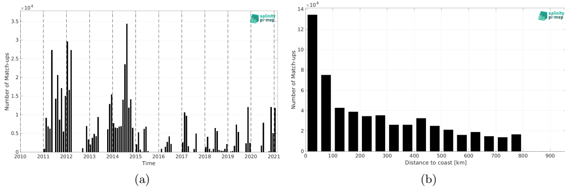
Figure 1: Number of match-ups between TSG (GOSUD-Sailing-ship) and SMOS SSS L4 v2 - Daily (BEC) SSS as a function of time (a) and as function of the distance to coast (b) over the SMOS coastal zone (<800km) 60N-60S Pi-MEP region and for the full satellite product period.
