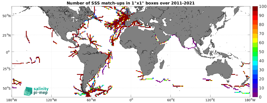
Figure 4: Number of SSS match-ups between TSG (GOSUD-Sailing-ship) SSS and the SMOS SSS L4 v2 - Daily (BEC) SSS product for the SMOS coastal zone (<800km) 60N-60S Pi-MEP region over 1^{\circ} \times 1^{\circ} boxes and for the full satellite product period.
