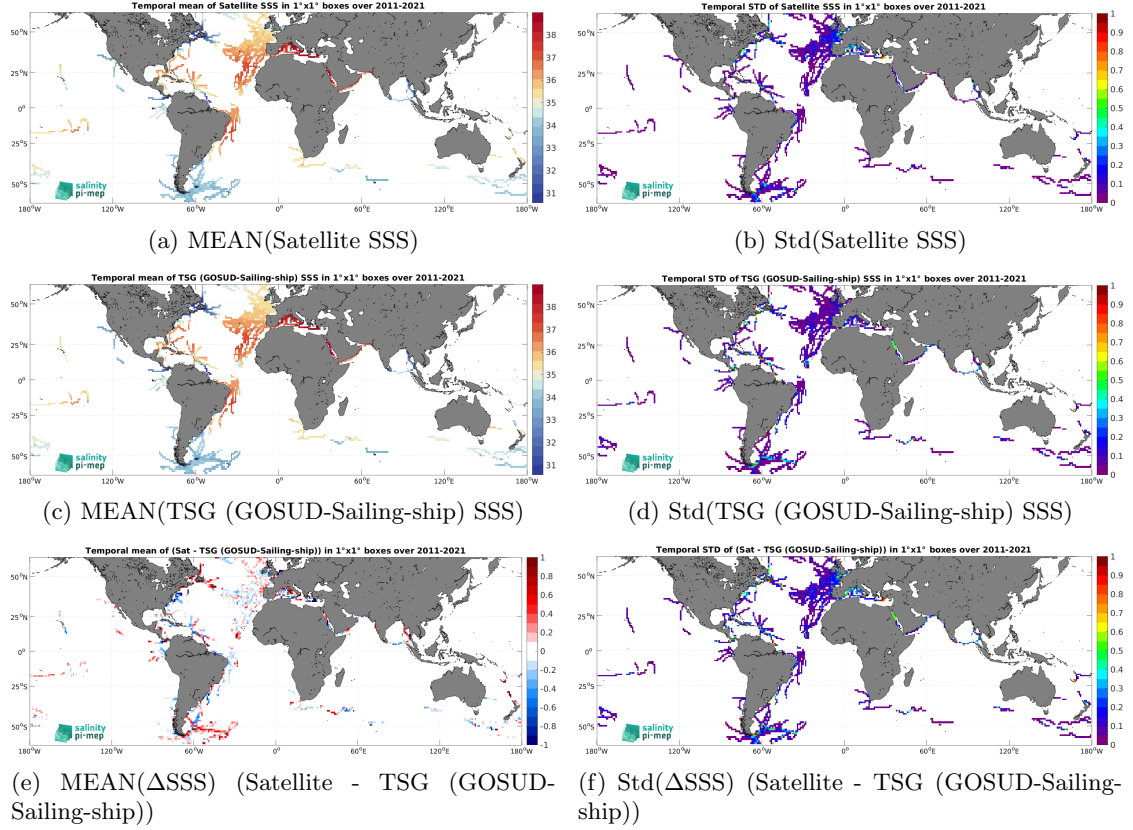
Figure 6: Temporal mean (left) and Std (right) of SSS from SMOS SSS L4 v2 - Daily (BEC) (top), TSG (GOSUD-Sailing-ship) (middle), and of \Delta SSS (Satellite - TSG (GOSUD-Sailing-ship)). Only match-up pairs are used to generate these maps.
