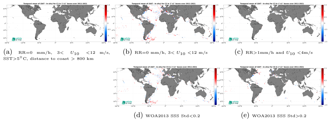
Figure 12: Temporal mean gridded over spatial boxes of size 1^\circ \times 1^\circ of \Delta\text{SSS} (SMOS SSS L4 v2 - Daily (BEC) - TSG (GOSUD-Sailing-ship)) for 5 different subdatasets corresponding to: RR=0 mm/h, 3 < U_{10} < 12 m/s, SST > 5°C, distance to coast > 800 km (a), RR=0 mm/h, 3 < U_{10} < 12 m/s (b), RR > 1mm/h and U_{10} < 4 m/s (c), WOA2013 SSS Std < 0.2 (d), WOA2013 SSS Std > 0.2 (e).
