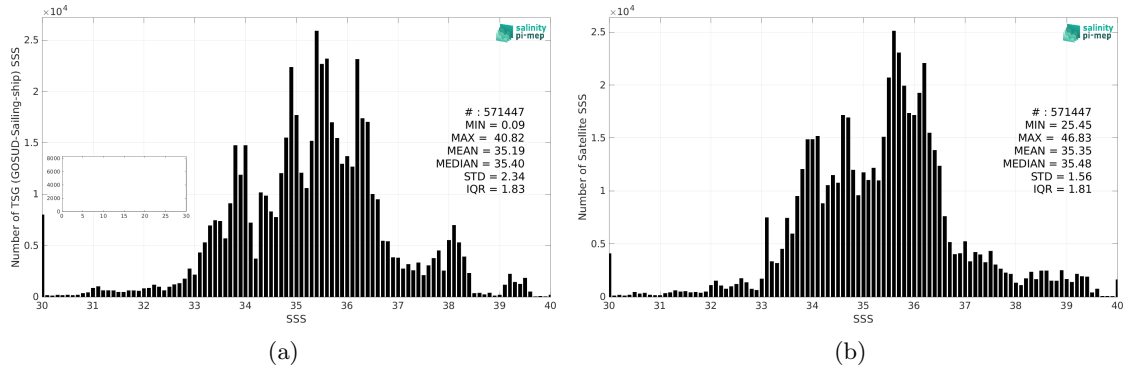
Figure 2: Histograms of SSS from TSG (GOSUD-Sailing-ship) (a) and SMOS SSS L4 v2 - Daily (BEC) (b) considering all match-up pairs per bins of 0.1 over the SMOS coastal zone (<800km) 60N-60S Pi-MEP region and for the full satellite product period.
