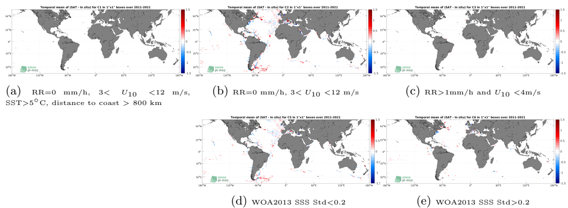
Figure 12: Temporal mean gridded over spatial boxes of size 1^\circ \times 1^\circ of \Delta SSS (SMOS SSS L4 v2 - Daily (BEC) - TSG (GOSUD-Sailing-ship)) for 5 different subdatasets corresponding to:RR=0 mm/h, 3 < U_{10} < 12 m/s, SST >5^\circ\text{C} , distance to coast > 800 km (a), RR=0 mm/h, 3 < U_{10} < 12 m/s (b), RR >1 mm/h and U_{10} < 4 m/s (c), WOA2013 SSS Std <0.2 (d), WOA2013 SSS Std >0.2 (e).
