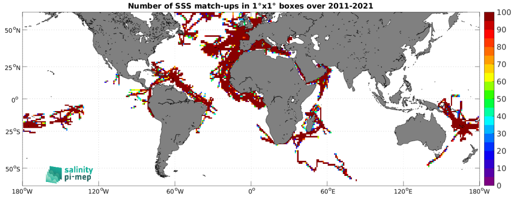
Figure 5: Number of SSS match-ups between TSG (GOSUD-Research-vessel) SSS and the SMOS SSS L4 v2 - Daily (BEC) SSS product for the SMOS coastal zone (<800km) 60N-60S Pi-MEP region over 1^\circ \times 1^\circ boxes and for the full satellite product period.
