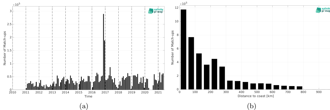
Figure 2: Number of match-ups between TSG (GOSUD-Research-vessel) and SMOS SSS L4 v2 - Daily (BEC) SSS as a function of time (a) and as function of the distance to coast (b) over the SMOS coastal zone (<800km) 60N-60S Pi-MEP region and for the full satellite product period.
