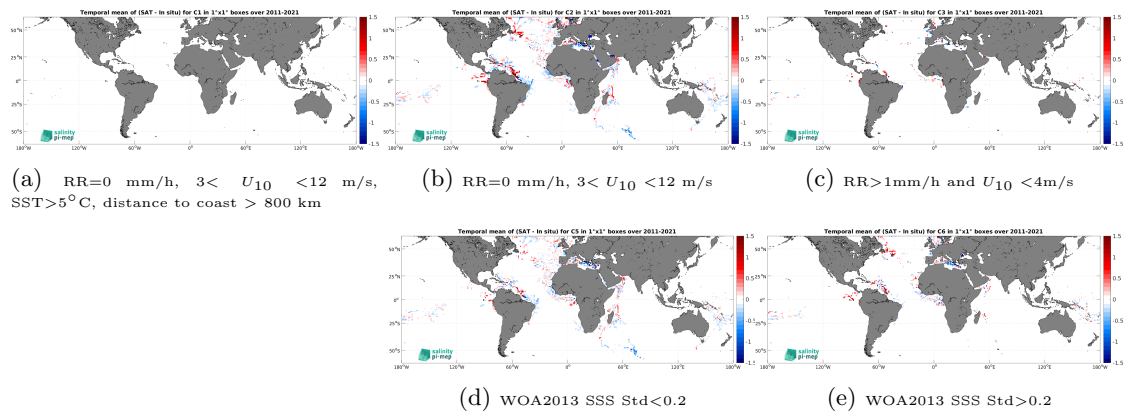
Figure 14: Temporal mean gridded over spatial boxes of size 1^\circ \times 1^\circ of \Delta\text{SSS} (SMOS SSS L4 v2 - Daily (BEC) - TSG (GOSUD-Research-vessel)) for 5 different subdatasets corresponding to:RR=0 mm/h, 3 < U_{10} < 12 m/s, SST >5^\circ\text{C} , distance to coast > 800 km (a), RR=0 mm/h, 3 < U_{10} < 12 m/s (b), RR >1 mm/h and U_{10} < 4 m/s (c), WOA2013 SSS Std <0.2 (d), WOA2013 SSS Std >0.2 (e).
