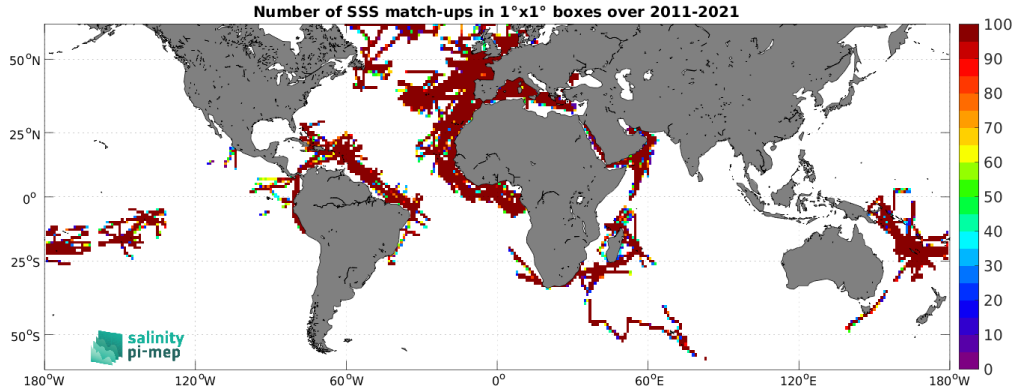
Figure 5: Number of SSS match-ups between TSG (GOSUD-Research-vessel) SSS and the SMOS SSS L4 v2 - Daily (BEC) SSS product for the SMOS coastal zone (<800km) 60N-60S Pi-MEP region over 1^{\circ} \times 1^{\circ} boxes and for the full satellite product period.
