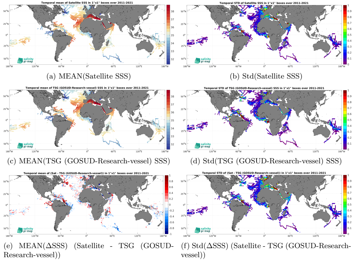
Figure 7: Temporal mean (left) and Std (right) of SSS from SMOS SSS L4 v2 - Daily (BEC) (top), TSG (GOSUD-Research-vessel) (middle), and of \Delta SSS (Satellite - TSG (GOSUD-Research-vessel)). Only match-up pairs are used to generate these maps.
