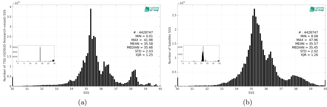
Figure 3: Histograms of SSS from TSG (GOSUD-Research-vessel) (a) and SMOS SSS L4 v2 - Daily (BEC) (b) considering all match-up pairs per bins of 0.1 over the SMOS coastal zone (<800km) 60N-60S Pi-MEP region and for the full satellite product period.
