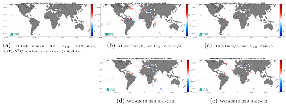
Figure 12: Temporal mean gridded over spatial boxes of size 1^\circ \times 1^\circ of \Delta\text{SSS} (SMOS SSS L4 v2 - Daily (BEC) - TSG (GOSUD-Research-vessel)) for 5 different subdatasets corresponding to:RR=0 mm/h, 3 < U_{10} < 12 m/s, SST >5^\circ\text{C} , distance to coast > 800 km (a), RR=0 mm/h, 3 < U_{10} < 12 m/s (b), RR >1 mm/h and U_{10} < 4 m/s (c), WOA2013 SSS Std <0.2 (d), WOA2013 SSS Std >0.2 (e).
