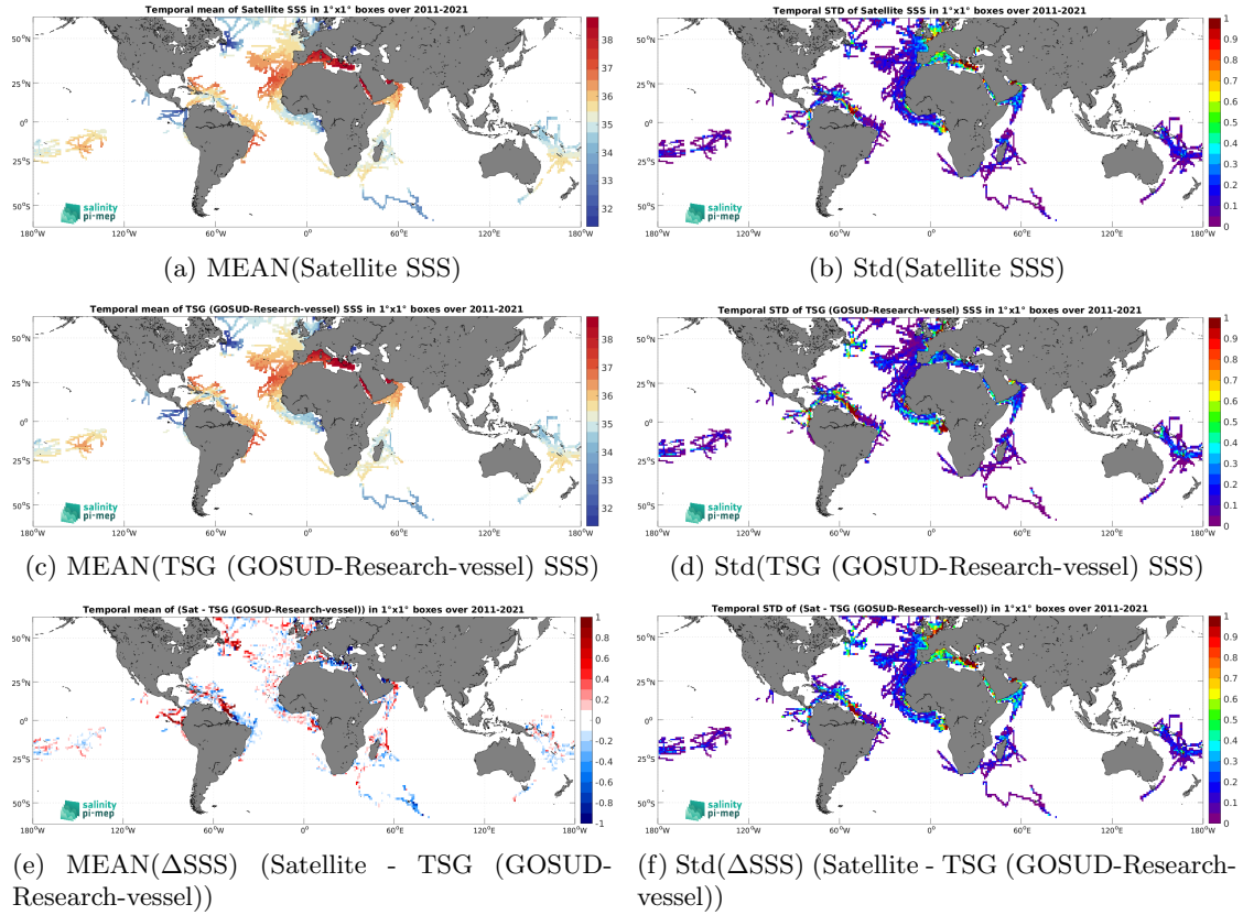
Figure 6: Temporal mean (left) and Std (right) of SSS from SMOS SSS L4 v2 - Daily (BEC) (top), TSG (GOSUD-Research-vessel) (middle), and of \Delta SSS (Satellite - TSG (GOSUD-Research-vessel)). Only match-up pairs are used to generate these maps.
