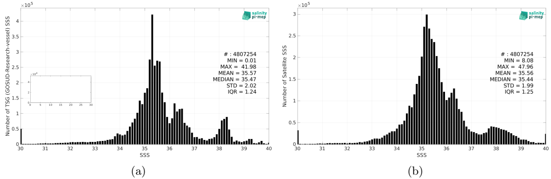
Figure 2: Histograms of SSS from TSG (GOSUD-Research-vessel) (a) and SMOS SSS L4 v2 - Daily (BEC) (b) considering all match-up pairs per bins of 0.1 over the SMOS coastal zone (<800km) 60N-60S Pi-MEP region and for the full satellite product period.
