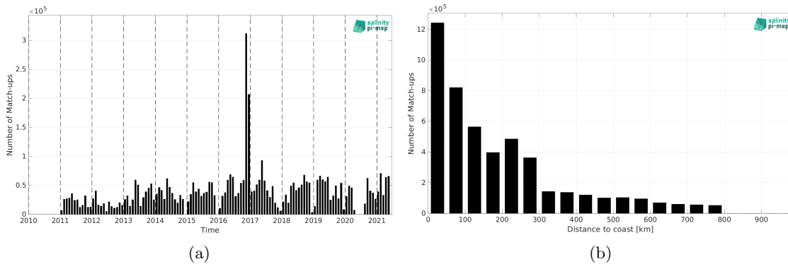
Figure 1: Number of match-ups between TSG (GOSUD-Research-vessel) and SMOS SSS L4 v2 - Daily (BEC) SSS as a function of time (a) and as function of the distance to coast (b) over the SMOS coastal zone (<800km) 60N-60S Pi-MEP region and for the full satellite product period.
