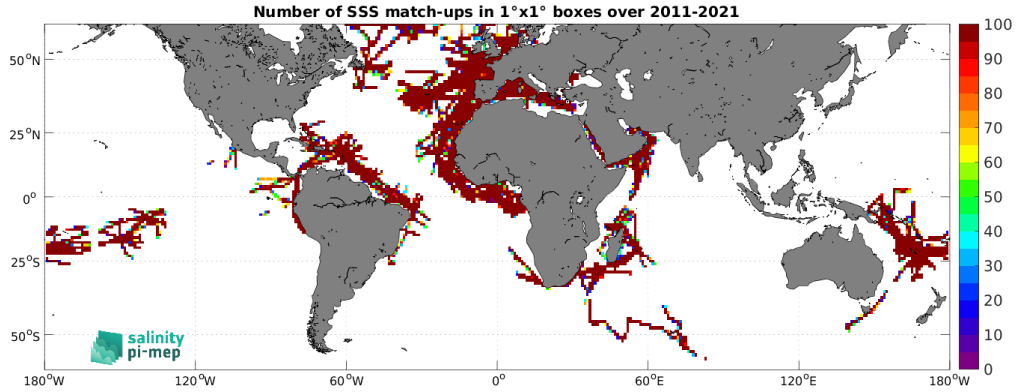
Figure 4: Number of SSS match-ups between TSG (GOSUD-Research-vessel) SSS and the SMOS SSS L4 v2 - Daily (BEC) SSS product for the SMOS coastal zone (<800km) 60N-60S Pi-MEP region over 1^\circ \times 1^\circ boxes and for the full satellite product period.
