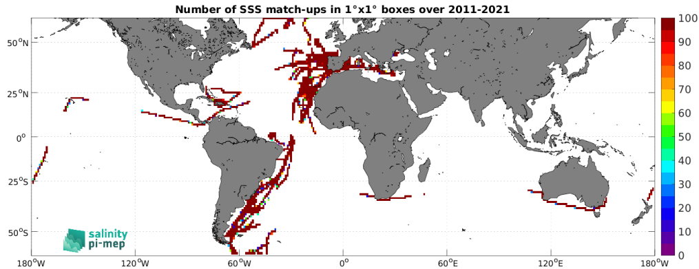
Figure 5: Number of SSS match-ups between TSG (CSIC-UTM) SSS and the SMOS SSS L4 v2 - Daily (BEC) SSS product for the SMOS coastal zone (<800km) 60N-60S Pi-MEP region over 1^\circ \times 1^\circ boxes and for the full satellite product period.
