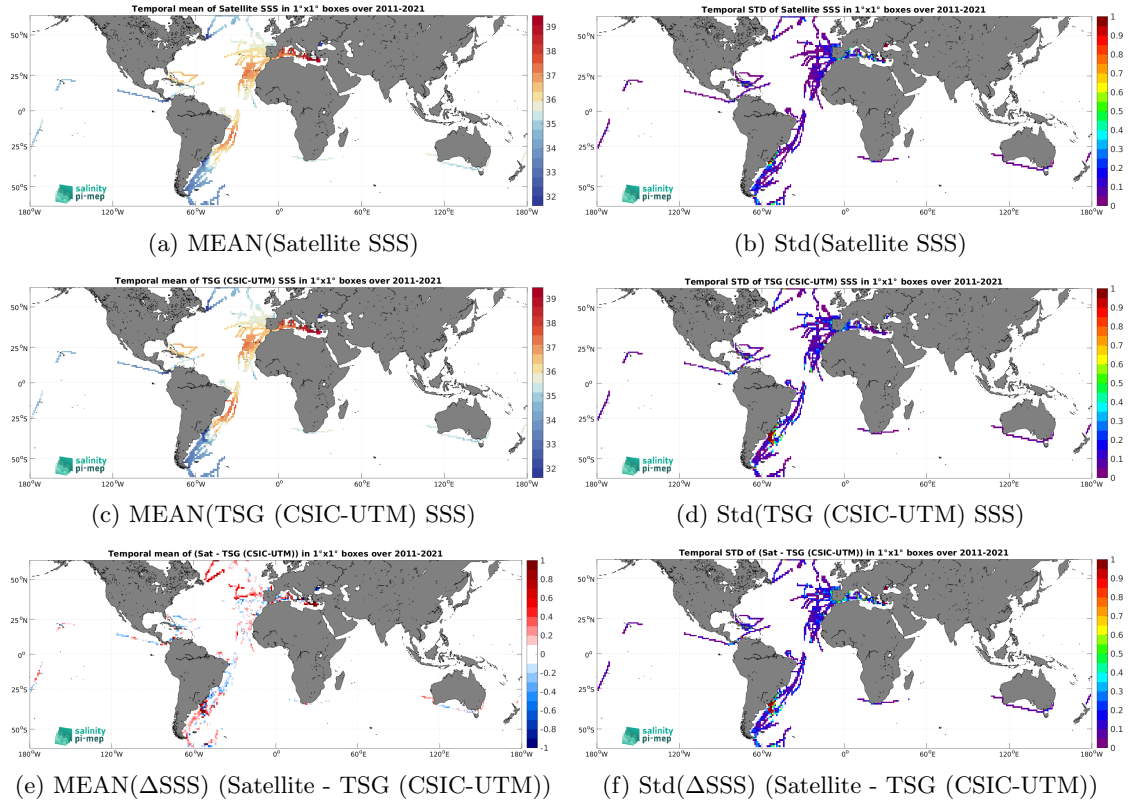
Figure 7: Temporal mean (left) and Std (right) of SSS from SMOS SSS L4 v2 - Daily (BEC) (top), TSG (CSIC-UTM) (middle), and of \Delta SSS (Satellite - TSG (CSIC-UTM)). Only match-up pairs are used to generate these maps.
