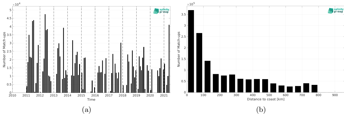
Figure 2: Number of match-ups between TSG (CSIC-UTM) and SMOS SSS L4 v2 - Daily (BEC) SSS as a function of time (a) and as function of the distance to coast (b) over the SMOS coastal zone (<800km) 60N-60S Pi-MEP region and for the full satellite product period.
