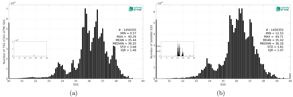
Figure 3: Histograms of SSS from TSG (CSIC-UTM) (a) and SMOS SSS L4 v2 - Daily (BEC) (b) considering all match-up pairs per bins of 0.1 over the SMOS coastal zone (<800km) 60N-60S Pi-MEP region and for the full satellite product period.
