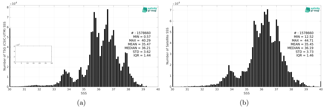
Figure 2: Histograms of SSS from TSG (CSIC-UTM) (a) and SMOS SSS L4 v2 - Daily (BEC) (b) considering all match-up pairs per bins of 0.1 over the SMOS coastal zone (<800km) 60N-60S Pi-MEP region and for the full satellite product period.
