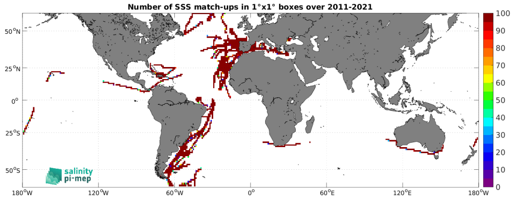
Figure 4: Number of SSS match-ups between TSG (CSIC-UTM) SSS and the SMOS SSS L4 v2 - Daily (BEC) SSS product for the SMOS coastal zone (<800km) 60N-60S Pi-MEP region over 1^\circ \times 1^\circ boxes and for the full satellite product period.
