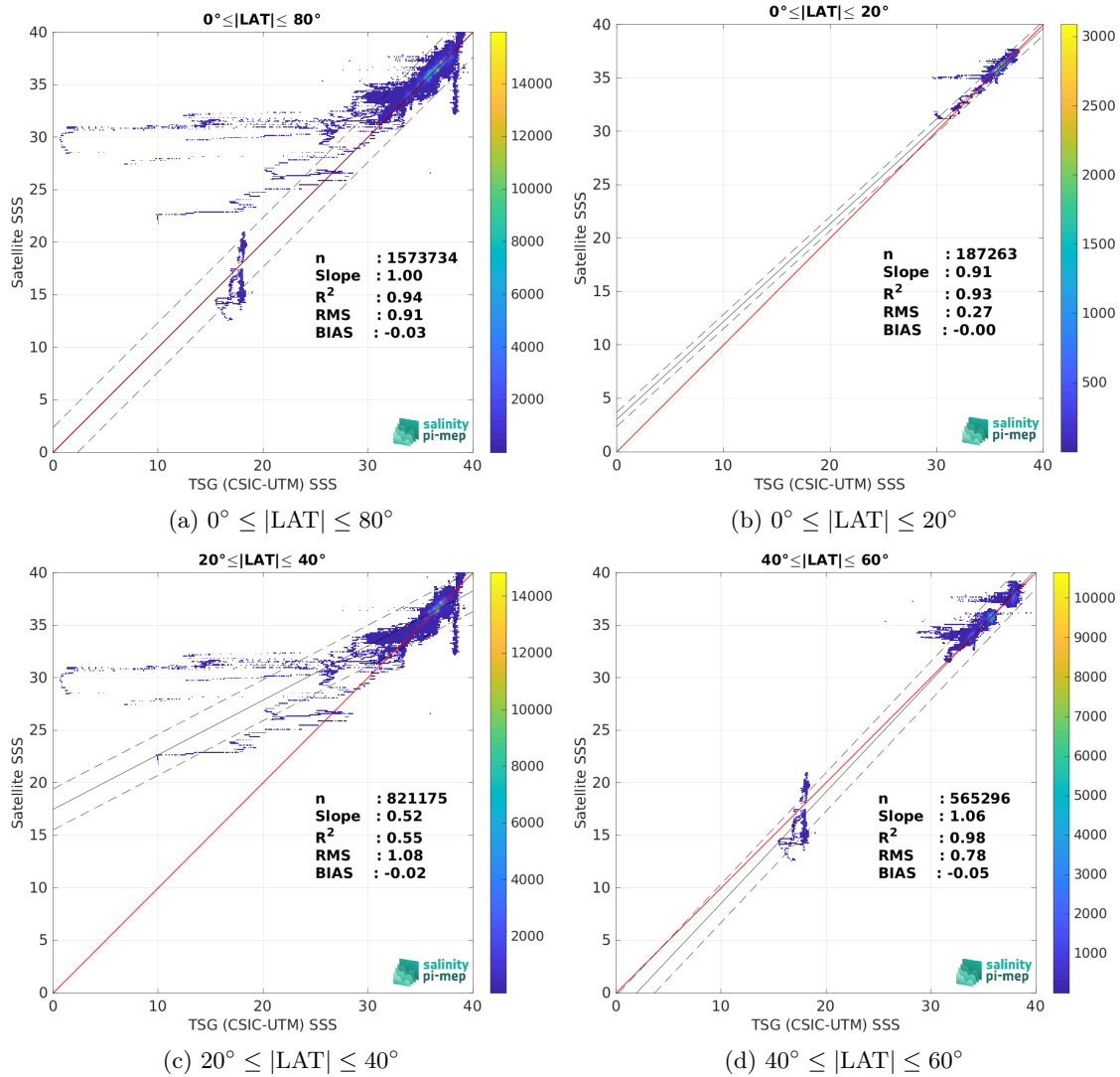
Figure 9: Contour maps of the concentration of SMOS SSS L4 v2 - Daily (BEC) SSS (y-axis) versus TSG (CSIC-UTM) SSS (x-axis) at match-up pairs for different latitude bands. For each plot, the red line shows x=y . The black thin and dashed lines indicate a linear fit through the data cloud and the \pm 95\% confidence levels, respectively. The number match-up pairs n , the slope and R^2 coefficient of the linear fit, the root mean square (RMS) and the mean bias between satellite and in situ data are indicated for each latitude band in each plots.
