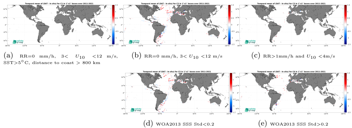
Figure 12: Temporal mean gridded over spatial boxes of size 1^\circ \times 1^\circ of \Delta\text{SSS} (SMOS SSS L4 v2 - Daily (BEC) - TSG (CSIC-UTM)) for 5 different subdatasets corresponding to:RR=0 mm/h, 3 < U_{10} < 12 m/s, SST >5^\circ\text{C} , distance to coast > 800 km (a), RR=0 mm/h, 3 < U_{10} < 12 m/s (b), RR >1 mm/h and U_{10} < 4 m/s (c), WOA2013 SSS Std <0.2 (d), WOA2013 SSS Std >0.2 (e).
