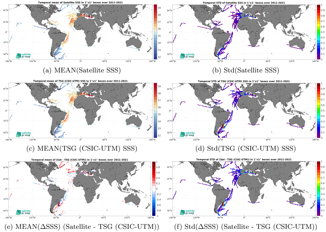
Figure 6: Temporal mean (left) and Std (right) of SSS from SMOS SSS L4 v2 - Daily (BEC) (top), TSG (CSIC-UTM) (middle), and of \Delta SSS (Satellite - TSG (CSIC-UTM)). Only match-up pairs are used to generate these maps.
