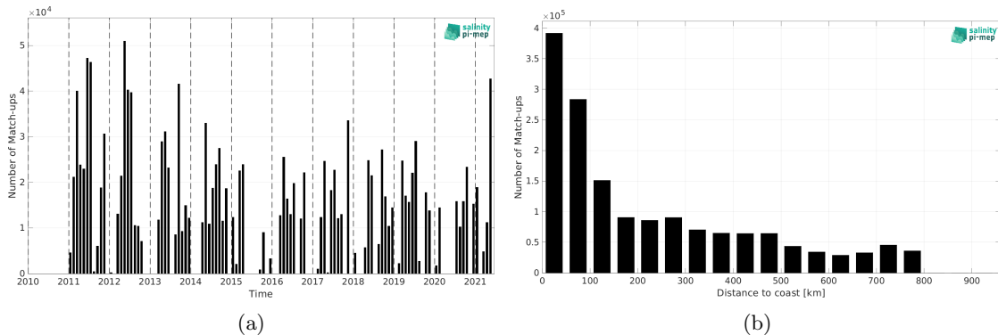
Figure 1: Number of match-ups between TSG (CSIC-UTM) and SMOS SSS L4 v2 - Daily (BEC) SSS as a function of time (a) and as function of the distance to coast (b) over the SMOS coastal zone (<800km) 60N-60S Pi-MEP region and for the full satellite product period.
