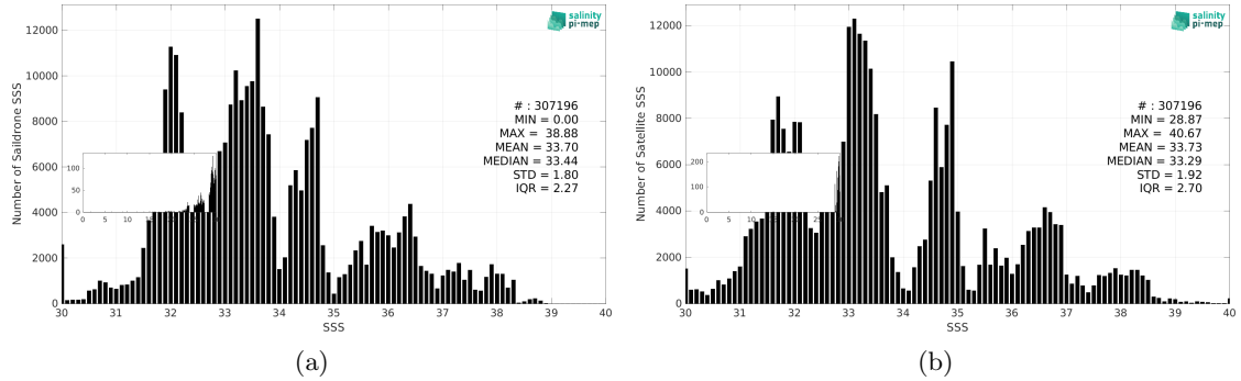
Figure 3: Histograms of SSS from Saildrone (a) and SMOS SSS L4 v2 - Daily (BEC) (b) considering all match-up pairs per bins of 0.1 over the SMOS coastal zone (<800km) 60N-60S Pi-MEP region and for the full satellite product period.
