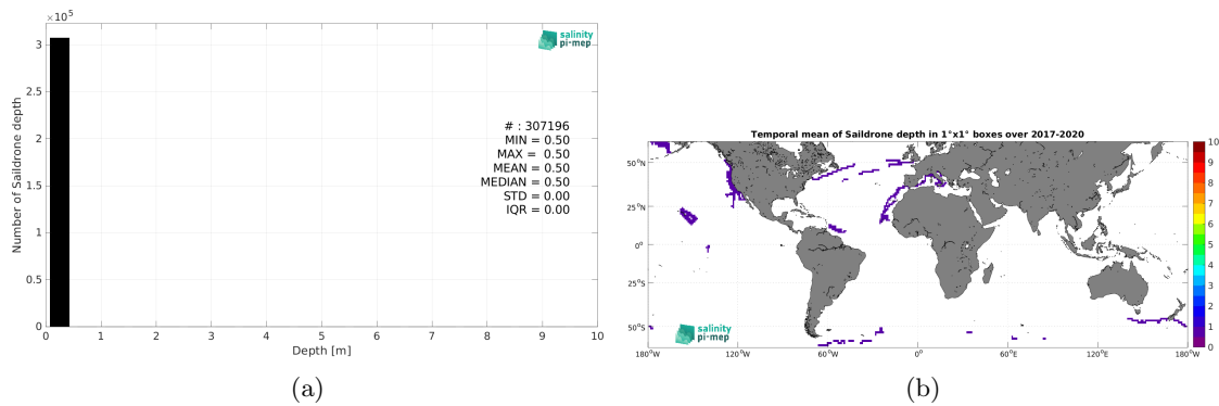
Figure 4: Histograms of the depth of the upper level SSS measurements from Sairdrone in the Match-up DataBase for the SMOS coastal zone (<800km) 60N-60S Pi-MEP region (a) and temporal mean spatial distribution of pressure of the in situ SSS data over 1^\circ \times 1^\circ boxes and for the full satellite product period (b).
