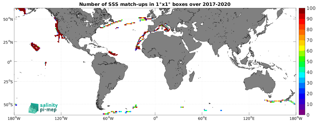
Figure 5: Number of SSS match-ups between Saildrone SSS and the SMOS SSS L4 v2 - Daily (BEC) SSS product for the SMOS coastal zone (<800km) 60N-60S Pi-MEP region over 1^\circ \times 1^\circ boxes and for the full satellite product period.
