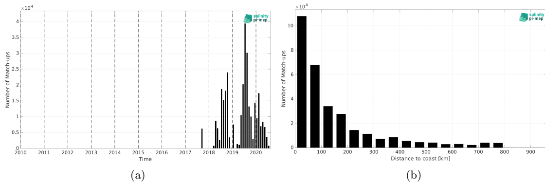
Figure 2: Number of match-ups between Saildrone and SMOS SSS L4 v2 - Daily (BEC) SSS as a function of time (a) and as function of the distance to coast (b) over the SMOS coastal zone (<800km) 60N-60S Pi-MEP region and for the full satellite product period.
