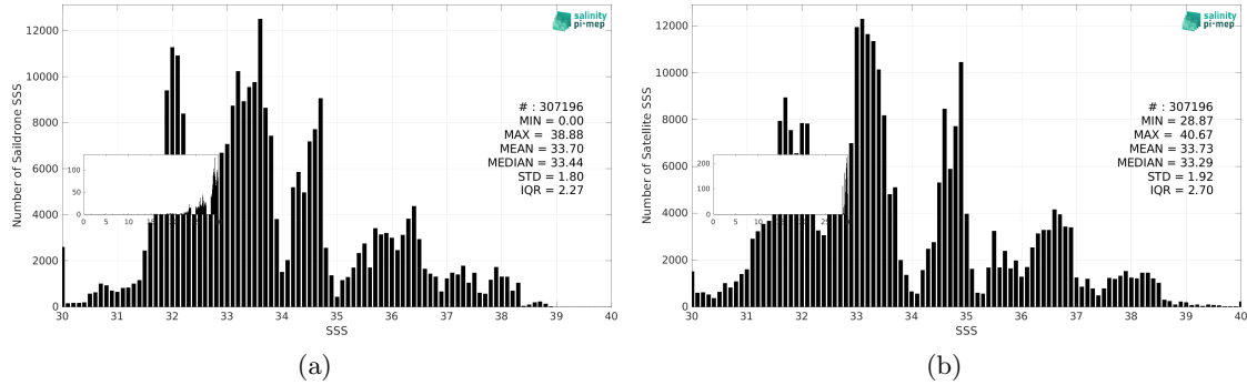
Figure 3: Histograms of SSS from Sairdrone (a) and SMOS SSS L4 v2 - Daily (BEC) (b) considering all match-up pairs per bins of 0.1 over the SMOS coastal zone (<800km) 60N-60S Pi-MEP region and for the full satellite product period.
