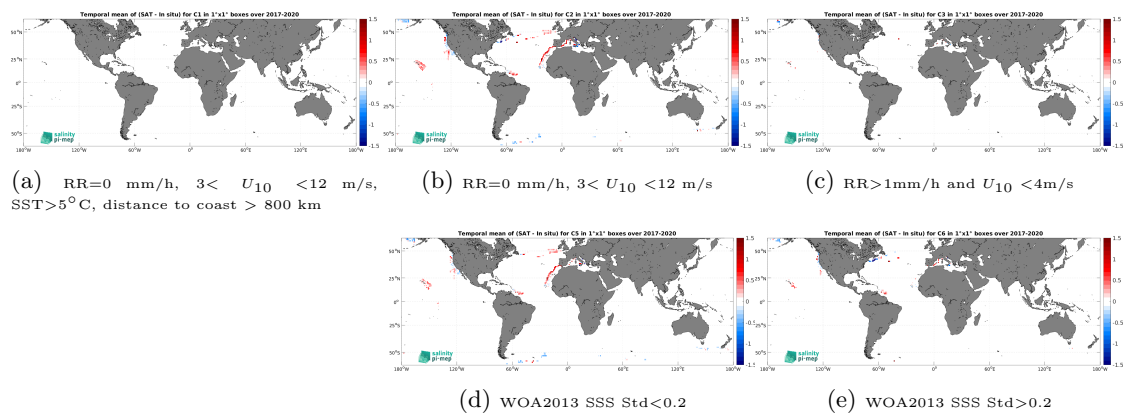
Figure 14: Temporal mean gridded over spatial boxes of size 1^\circ \times 1^\circ of \Delta SSS (SMOS SSS L4 v2 - Daily (BEC) - Saldrone) for 5 different subdatasets corresponding to:RR=0 mm/h, 3 < U_{10} < 12 m/s, SST >5^\circ\text{C} , distance to coast > 800 km (a), RR=0 mm/h, 3 < U_{10} < 12 m/s (b), RR >1 mm/h and U_{10} < 4 m/s (c), WOA2013 SSS Std <0.2 (d), WOA2013 SSS Std >0.2 (e).
