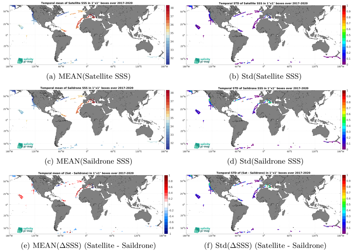
Figure 7: Temporal mean (left) and Std (right) of SSS from SMOS SSS L4 v2 - Daily (BEC) (top), Saildrone (middle), and of \Delta SSS (Satellite - Saildrone). Only match-up pairs are used to generate these maps.
