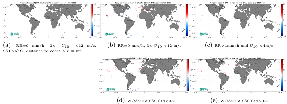
Figure 12: Temporal mean gridded over spatial boxes of size 1^\circ \times 1^\circ of \Delta\text{SSS} (SMOS SSS L4 v2 - Daily (BEC) - Saldrone) for 5 different subdatasets corresponding to:RR=0 mm/h, 3 < U_{10} < 12 m/s, SST >5^\circ\text{C} , distance to coast > 800 km (a), RR=0 mm/h, 3 < U_{10} < 12 m/s (b), RR >1 mm/h and U_{10} < 4 m/s (c), WOA2013 SSS Std <0.2 (d), WOA2013 SSS Std >0.2 (e).
