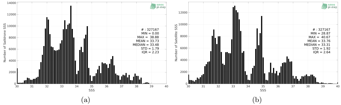
Figure 2: Histograms of SSS from Saildrone (a) and SMOS SSS L4 v2 - Daily (BEC) (b) considering all match-up pairs per bins of 0.1 over the SMOS coastal zone (<800km) 60N-60S Pi-MEP region and for the full satellite product period.
