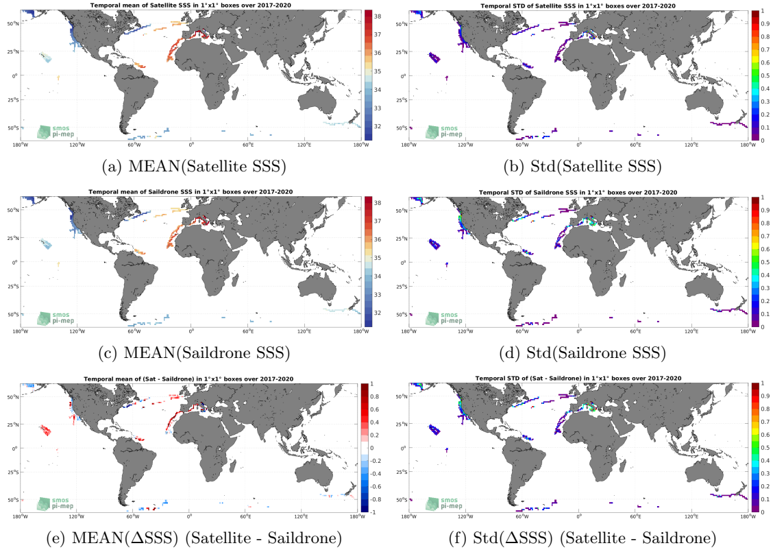
Figure 6: Temporal mean (left) and Std (right) of SSS from SMOS SSS L4 v2 - Daily (BEC) (top), Saildrone (middle), and of \Delta SSS (Satellite - Saildrone). Only match-up pairs are used to generate these maps.
