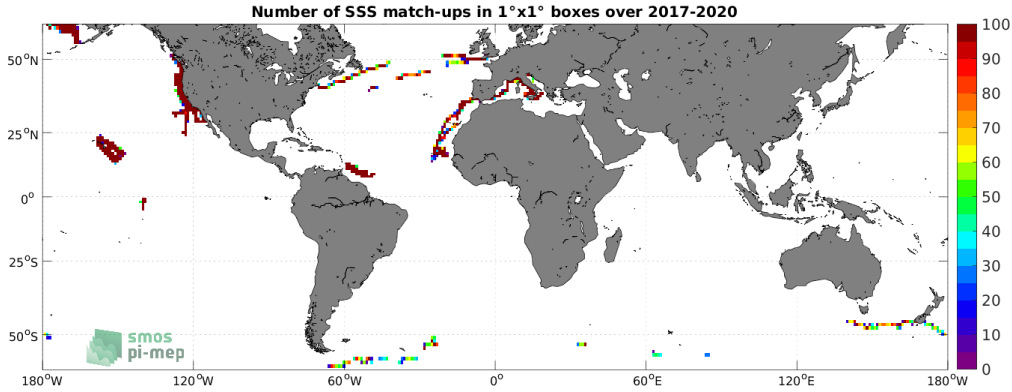
Figure 4: Number of SSS match-ups between Saildrone SSS and the SMOS SSS L4 v2 - Daily (BEC) SSS product for the SMOS coastal zone ( <800\text{km} ) 60N-60S Pi-MEP region over 1^\circ \times 1^\circ boxes and for the full satellite product period.
