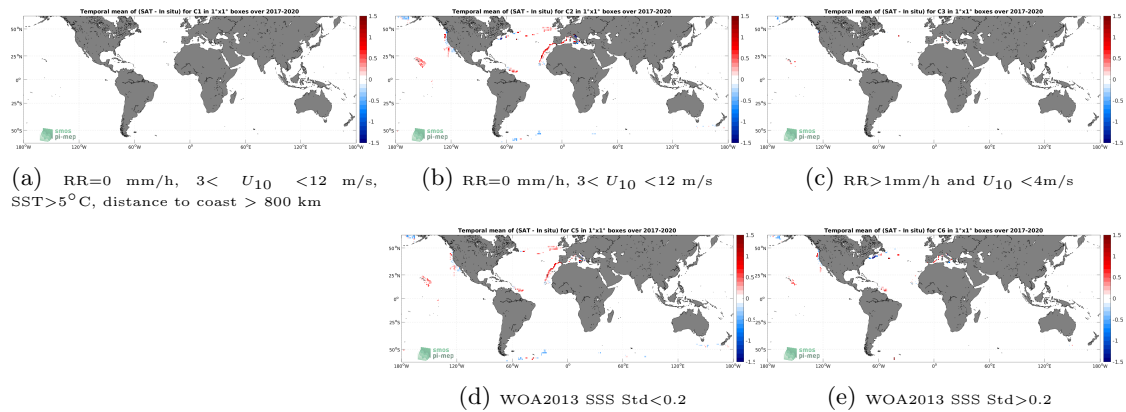
Figure 12: Temporal mean gridded over spatial boxes of size 1^\circ \times 1^\circ of \Delta SSS (SMOS SSS L4 v2 - Daily (BEC) - Saldrone) for 5 different subdatasets corresponding to:RR=0 mm/h, 3 < U_{10} < 12 m/s, SST >5^\circ\text{C} , distance to coast > 800 km (a), RR=0 mm/h, 3 < U_{10} < 12 m/s (b), RR >1 mm/h and U_{10} < 4 m/s (c), WOA2013 SSS Std <0.2 (d), WOA2013 SSS Std >0.2 (e).
