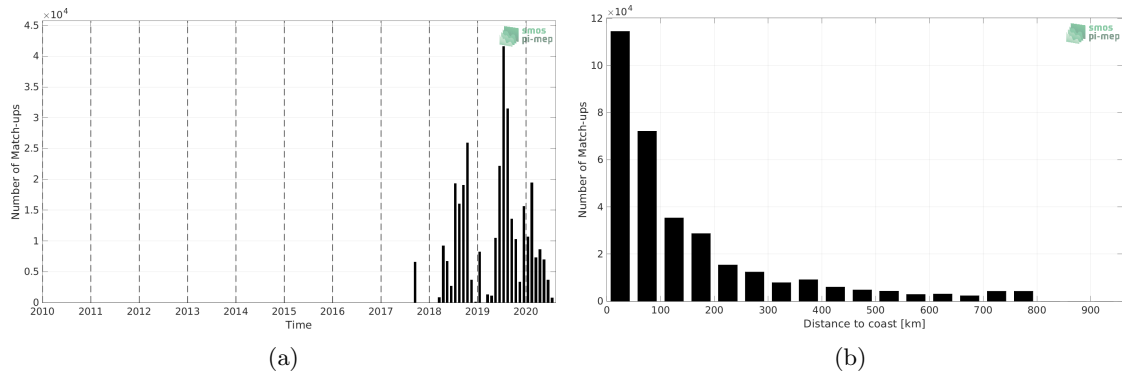
Figure 1: Number of match-ups between Saildrone and SMOS SSS L4 v2 - Daily (BEC) SSS as a function of time (a) and as function of the distance to coast (b) over the SMOS coastal zone (<800km) 60N-60S Pi-MEP region and for the full satellite product period.
