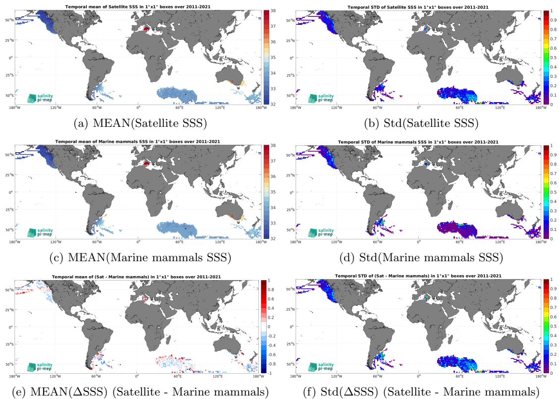
Figure 7: Temporal mean (left) and Std (right) of SSS from SMOS SSS L4 v2 - Daily (BEC) (top), Marine mammals (middle), and of \Delta SSS (Satellite - Marine mammals). Only match-up pairs are used to generate these maps.
