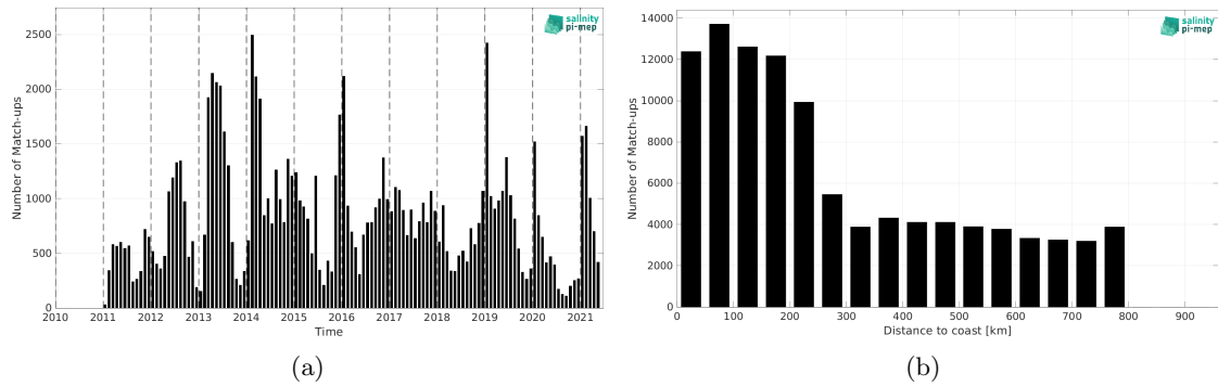
Figure 2: Number of match-ups between Marine mammals and SMOS SSS L4 v2 - Daily (BEC) SSS as a function of time (a) and as function of the distance to coast (b) over the SMOS coastal zone (<800km) 60N-60S Pi-MEP region and for the full satellite product period.
