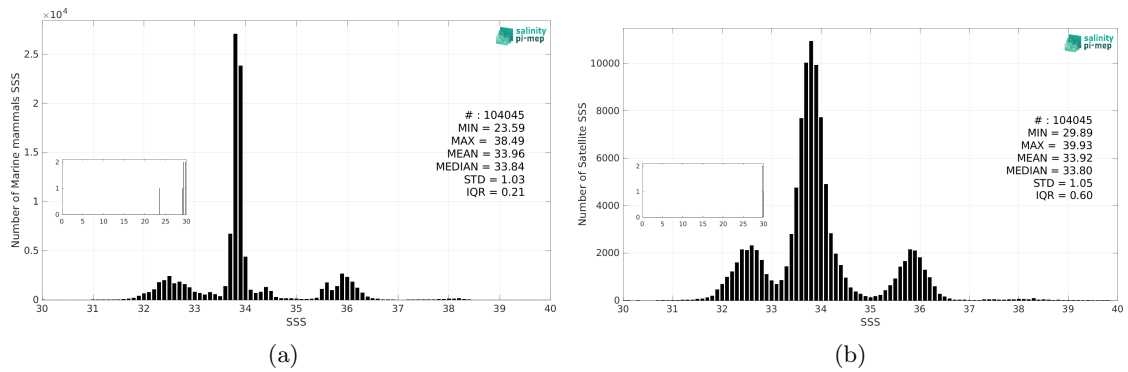
Figure 3: Histograms of SSS from Marine mammals (a) and SMOS SSS L4 v2 - Daily (BEC) (b) considering all match-up pairs per bins of 0.1 over the SMOS coastal zone (<800km) 60N-60S Pi-MEP region and for the full satellite product period.
