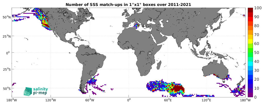
Figure 5: Number of SSS match-ups between Marine mammals SSS and the SMOS SSS L4 v2 - Daily (BEC) SSS product for the SMOS coastal zone (<800km) 60N-60S Pi-MEP region over 1^\circ \times 1^\circ boxes and for the full satellite product period.
