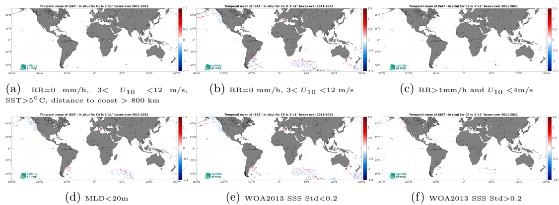
Figure 14: Temporal mean gridded over spatial boxes of size 1^\circ \times 1^\circ of \Delta SSS (SMOS SSS L4 v2 - Daily (BEC) - Marine mammals) for 6 different subdatasets corresponding to:RR=0 mm/h, 3 < U_{10} < 12 m/s, SST > 5^\circ\text{C} , distance to coast > 800 km (a), RR=0 mm/h, 3 < U_{10} < 12 m/s (b), RR > 1 mm/h and U_{10} < 4 m/s (c),MLD < 20 m (d),WOA2013 SSS Std < 0.2 (e),WOA2013 SSS Std > 0.2 (f).
