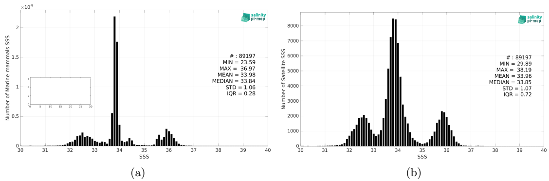
Figure 2: Histograms of SSS from Marine mammals (a) and SMOS SSS L4 v2 - Daily (BEC) (b) considering all match-up pairs per bins of 0.1 over the SMOS coastal zone (<800km) 60N-60S Pi-MEP region and for the full satellite product period.
