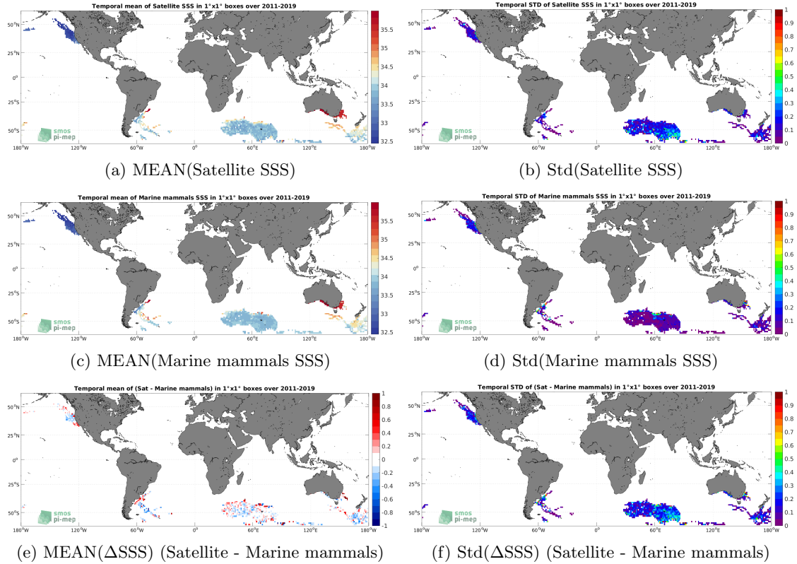
Figure 6: Temporal mean (left) and Std (right) of SSS from SMOS SSS L4 v2 - Daily (BEC) (top), Marine mammals (middle), and of \Delta SSS (Satellite - Marine mammals). Only match-up pairs are used to generate these maps.
