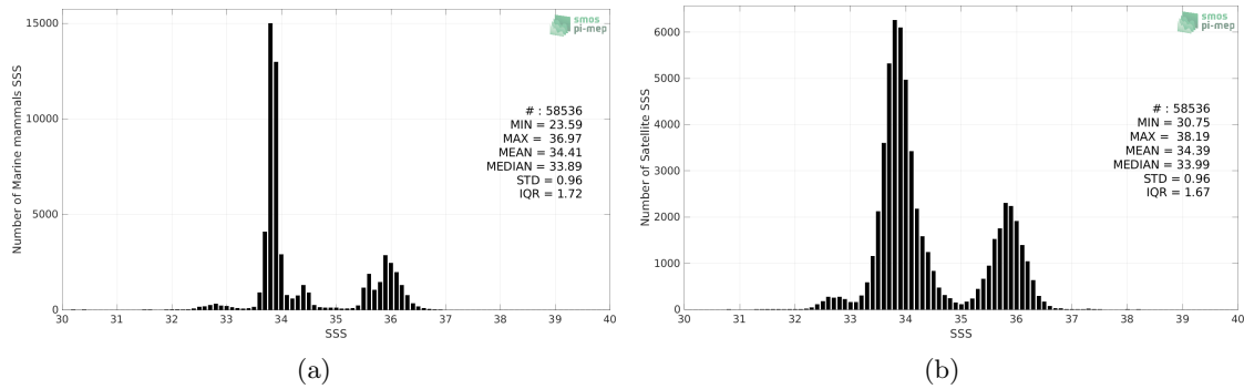
Figure 2: Histograms of SSS from Marine mammals (a) and SMOS SSS L4 v2 - Daily (BEC) (b) considering all match-up pairs per bins of 0.1 over the SMOS coastal zone (<800km) 60N-60S Pi-MEP region and for the full satellite product period.
