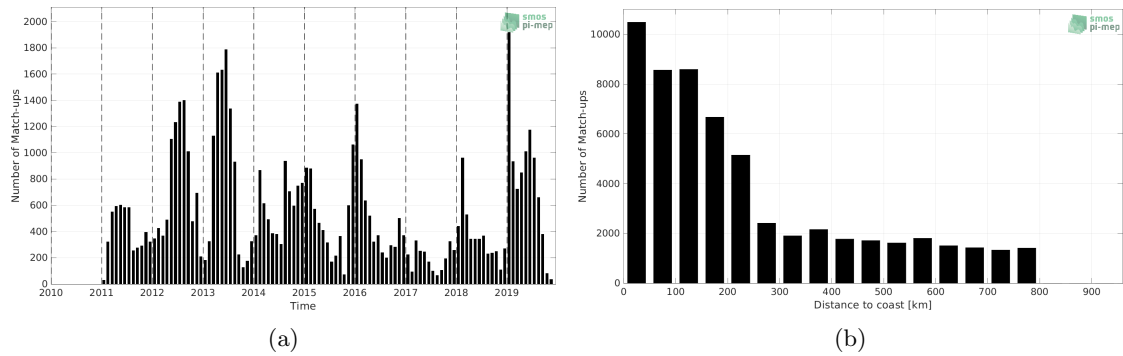
Figure 1: Number of match-ups between Marine mammals and SMOS SSS L4 v2 - Daily (BEC) SSS as a function of time (a) and as function of the distance to coast (b) over the SMOS coastal zone (<800km) 60N-60S Pi-MEP region and for the full satellite product period.
