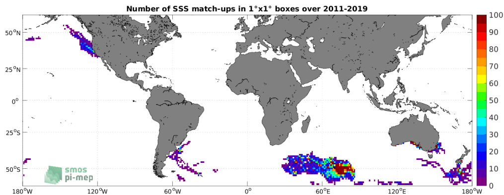
Figure 4: Number of SSS match-ups between Marine mammals SSS and the SMOS SSS L4 v2 - Daily (BEC) SSS product for the SMOS coastal zone (<800km) 60N-60S Pi-MEP region over 1^\circ \times 1^\circ boxes and for the full satellite product period.
