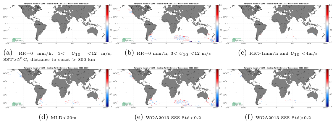
Figure 12: Temporal mean gridded over spatial boxes of size 1^\circ \times 1^\circ of \Delta SSS (SMOS SSS L4 v2 - Daily (BEC) - Marine mammals) for 6 different subdatasets corresponding to:RR=0 mm/h, 3 < U_{10} < 12 m/s, SST >5^\circ C, distance to coast > 800 km (a), RR=0 mm/h, 3 < U_{10} < 12 m/s (b), RR >1 mm/h and U_{10} < 4 m/s (c),MLD <20 m (d),WOA2013 SSS Std <0.2 (e),WOA2013 SSS Std >0.2 (f).
