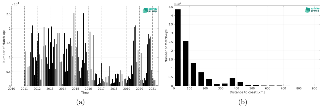
Figure 2: Number of match-ups between ICES and SMOS SSS L4 v2 - Daily (BEC) SSS as a function of time (a) and as function of the distance to coast (b) over the SMOS coastal zone ( < 800\text{km} ) 60N-60S Pi-MEP region and for the full satellite product period.
