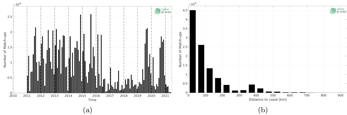
Figure 1: Number of match-ups between ICES and SMOS SSS L4 v2 - Daily (BEC) SSS as a function of time (a) and as function of the distance to coast (b) over the SMOS coastal zone (<800km) 60N-60S Pi-MEP region and for the full satellite product period.
