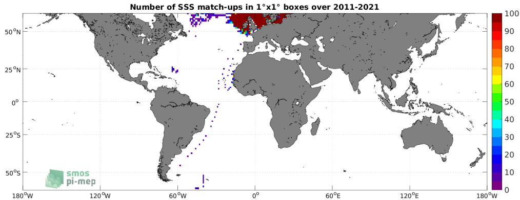
Figure 4: Number of SSS match-ups between ICES SSS and the SMOS SSS L4 v2 - Daily (BEC) SSS product for the SMOS coastal zone (<800km) 60N-60S Pi-MEP region over 1^\circ \times 1^\circ boxes and for the full satellite product period.
