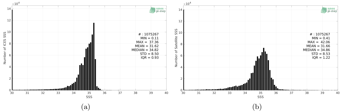
Figure 2: Histograms of SSS from ICES (a) and SMOS SSS L4 v2 - Daily (BEC) (b) considering all match-up pairs per bins of 0.1 over the SMOS coastal zone (<800km) 60N-60S Pi-MEP region and for the full satellite product period.
