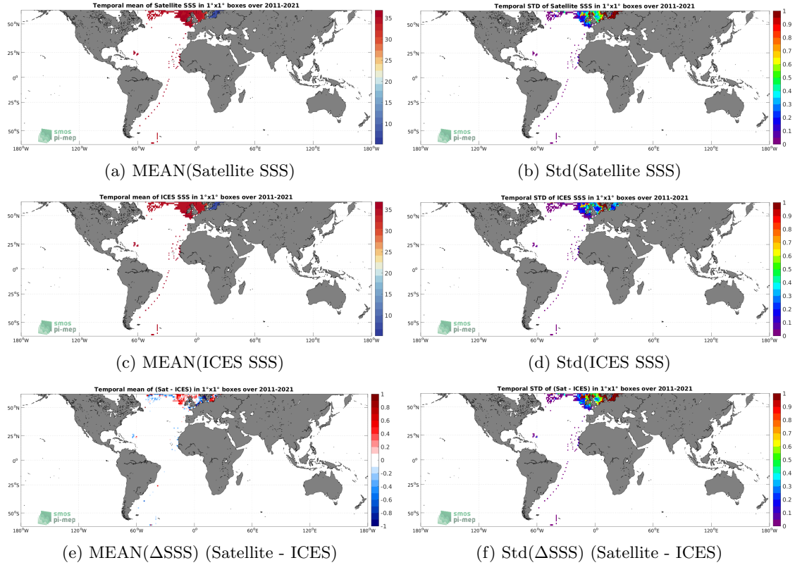
Figure 6: Temporal mean (left) and Std (right) of SSS from SMOS SSS L4 v2 - Daily (BEC) (top), ICES (middle), and of \Delta SSS (Satellite - ICES). Only match-up pairs are used to generate these maps.
