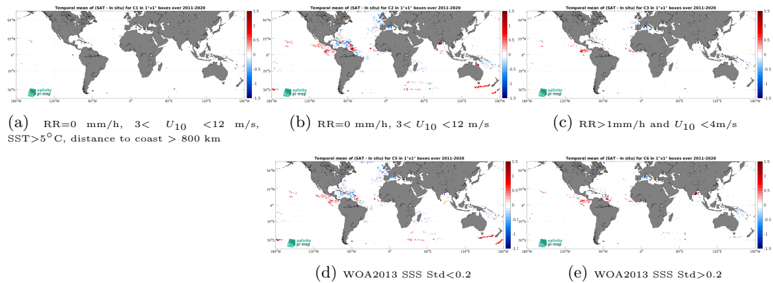
Figure 13: Temporal mean gridded over spatial boxes of size 1^\circ \times 1^\circ of \Delta SSS (SMOS SSS L4 v2 - Daily (BEC) - Surface drifters) for 5 different subdatasets corresponding to:RR=0 mm/h, 3 < U_{10} < 12 m/s, SST >5^\circ\text{C} , distance to coast > 800 km (a), RR=0 mm/h, 3 < U_{10} < 12 m/s (b), RR >1 mm/h and U_{10} < 4 m/s (c), WOA2013 SSS Std <0.2 (d), WOA2013 SSS Std >0.2 (e).
