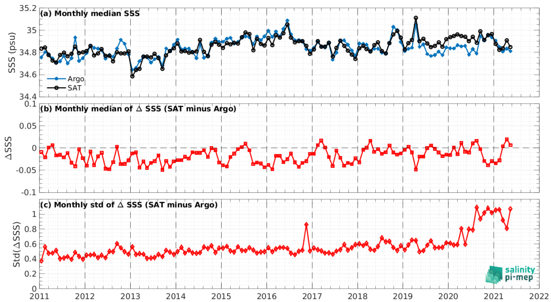
Figure 8: Time series of the monthly median SSS (top), median of \Delta SSS (Satellite - Argo) and Std of \Delta SSS (Satellite - Argo) over the SMOS coastal zone ( <800\text{km} ) 60\text{N} - 60\text{S} Pi-MEP region considering all match-ups collected by the Pi-MEP.
