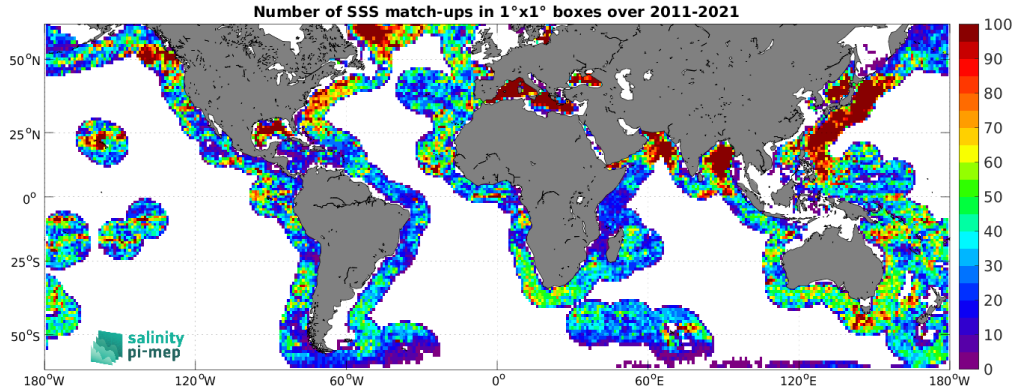
Figure 5: Number of SSS match-ups between Argo SSS and the SMOS SSS L4 v2 - Daily (BEC) SSS product for the SMOS coastal zone (<800km) 60N-60S Pi-MEP region over 1^\circ \times 1^\circ boxes and for the full satellite product period.
