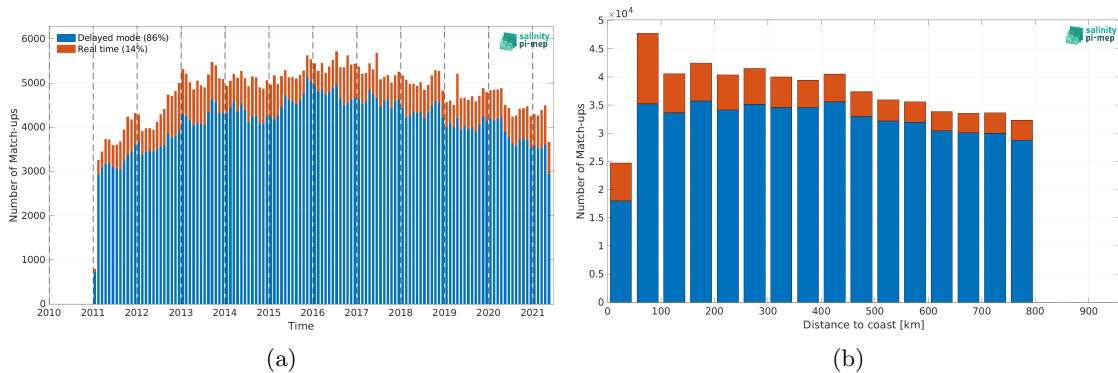
Figure 2: Number of match-ups between Argo and SMOS SSS L4 v2 - Daily (BEC) SSS as a function of time (a) and as function of the distance to coast (b) over the SMOS coastal zone ( < 800\text{km} ) 60\text{N}-60\text{S} Pi-MEP region and for the full satellite product period.
