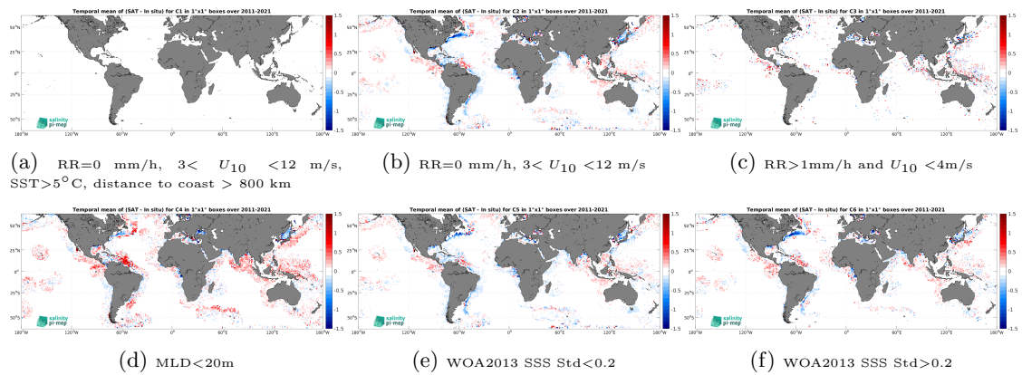
Figure 14: Temporal mean gridded over spatial boxes of size 1^\circ \times 1^\circ of \Delta SSS (SMOS SSS L4 v2 - Daily (BEC) - Argo) for 6 different subdatasets corresponding to:RR=0 mm/h, 3 < U_{10} < 12 m/s, SST > 5^\circ\text{C} , distance to coast > 800 km (a), RR=0 mm/h, 3 < U_{10} < 12 m/s (b), RR > 1 mm/h and U_{10} < 4 m/s (c),MLD < 20 m (d),WOA2013 SSS Std < 0.2 (e),WOA2013 SSS Std > 0.2 (f).
