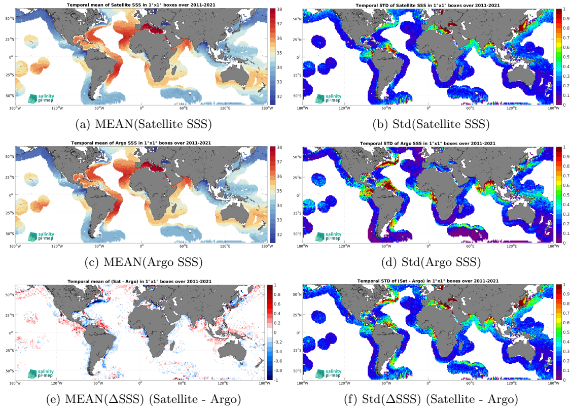
Figure 7: Temporal mean (left) and Std (right) of SSS from SMOS SSS L4 v2 - Daily (BEC) (top), Argo (middle), and of \Delta SSS (Satellite - Argo). Only match-up pairs are used to generate these maps.
