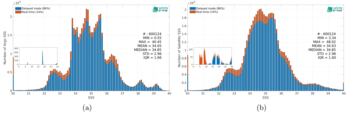
Figure 3: Histograms of SSS from Argo (a) and SMOS SSS L4 v2 - Daily (BEC) (b) considering all match-up pairs per bins of 0.1 over the SMOS coastal zone (<800km) 60N-60S Pi-MEP region and for the full satellite product period.
