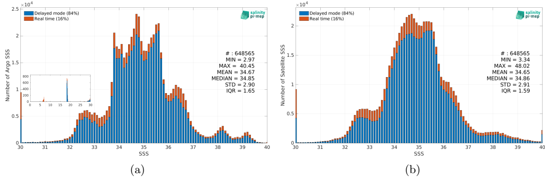
Figure 2: Histograms of SSS from Argo (a) and SMOS SSS L4 v2 - Daily (BEC) (b) considering all match-up pairs per bins of 0.1 over the SMOS coastal zone (<800km) 60N-60S Pi-MEP region and for the full satellite product period.
