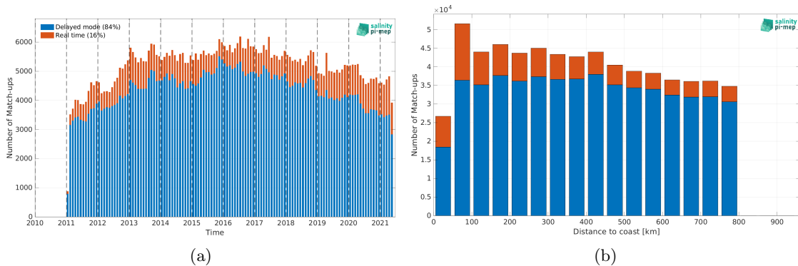
Figure 1: Number of match-ups between Argo and SMOS SSS L4 v2 - Daily (BEC) SSS as a function of time (a) and as function of the distance to coast (b) over the SMOS coastal zone ( < 800\text{km} ) 60\text{N}-60\text{S} Pi-MEP region and for the full satellite product period.
