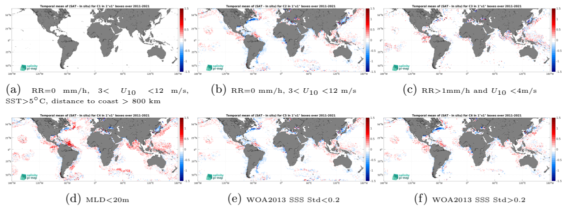
Figure 12: Temporal mean gridded over spatial boxes of size 1^\circ \times 1^\circ of \Delta SSS (SMOS SSS L4 v2 - Daily (BEC) - Argo) for 6 different subdatasets corresponding to:RR=0 mm/h, 3 < U_{10} < 12 m/s, SST > 5^\circ\text{C} , distance to coast > 800 km (a), RR=0 mm/h, 3 < U_{10} < 12 m/s (b), RR > 1 mm/h and U_{10} < 4 m/s (c),MLD < 20 m (d),WOA2013 SSS Std < 0.2 (e),WOA2013 SSS Std > 0.2 (f).
