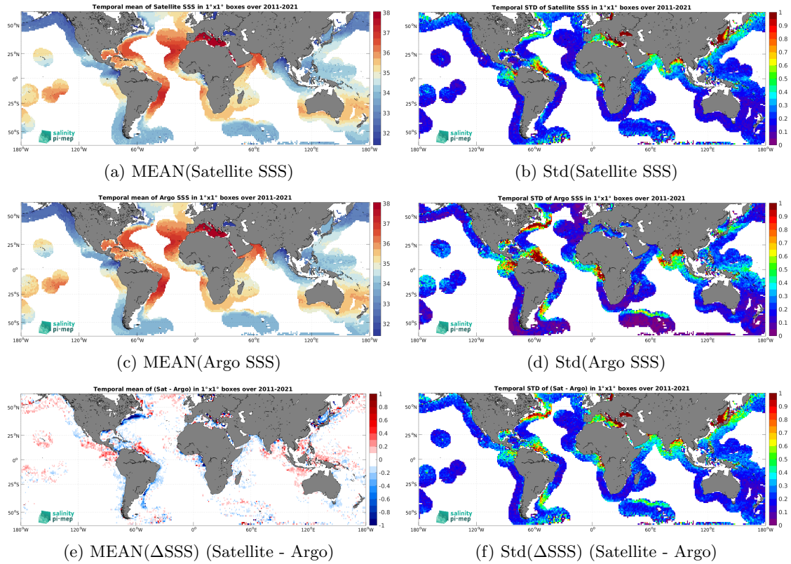
Figure 6: Temporal mean (left) and Std (right) of SSS from SMOS SSS L4 v2 - Daily (BEC) (top), Argo (middle), and of \Delta SSS (Satellite - Argo). Only match-up pairs are used to generate these maps.
