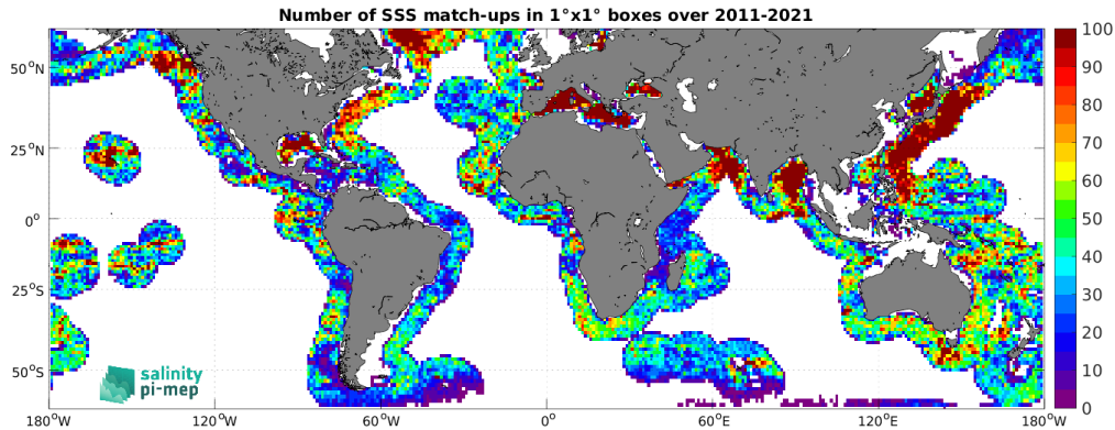
Figure 4: Number of SSS match-ups between Argo SSS and the SMOS SSS L4 v2 - Daily (BEC) SSS product for the SMOS coastal zone (<800km) 60N-60S Pi-MEP region over 1^\circ \times 1^\circ boxes and for the full satellite product period.
