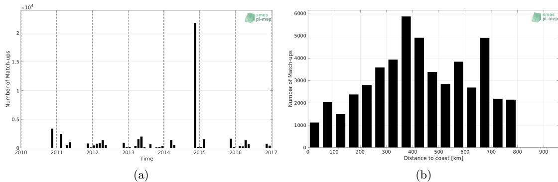
Figure 1: Number of match-ups between TSG (Polarstern) and SMOS SSS L3 v3 Monthly (ICDC) SSS as a function of time (a) and as function of the distance to coast (b) over the SMOS coastal zone (<800km) 60N-60S Pi-MEP region and for the full satellite product period.
