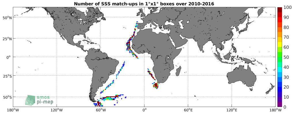
Figure 4: Number of SSS match-ups between TSG (Polarstern) SSS and the SMOS SSS L3 v3 Monthly (ICDC) SSS product for the SMOS coastal zone (<800km) 60N-60S Pi-MEP region over 1^\circ \times 1^\circ boxes and for the full satellite product period.
