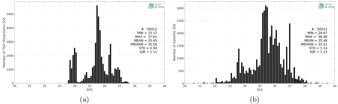
Figure 2: Histograms of SSS from TSG (Polarstern) (a) and SMOS SSS L3 v3 Monthly (ICDC) (b) considering all match-up pairs per bins of 0.1 over the SMOS coastal zone (<800km) 60N-60S Pi-MEP region and for the full satellite product period.
