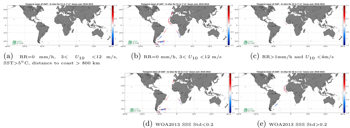
Figure 12: Temporal mean gridded over spatial boxes of size 1^\circ \times 1^\circ of \Delta\text{SSS} (SMOS SSS L3 v3 Monthly (ICDC) - TSG (Polarstern)) for 5 different subdatasets corresponding to:RR=0 mm/h, 3 < U_{10} < 12 m/s, SST >5^\circ\text{C} , distance to coast > 800 km (a), RR=0 mm/h, 3 < U_{10} < 12 m/s (b), RR >1 mm/h and U_{10} < 4 m/s (c), WOA2013 SSS Std <0.2 (d), WOA2013 SSS Std >0.2 (e).
