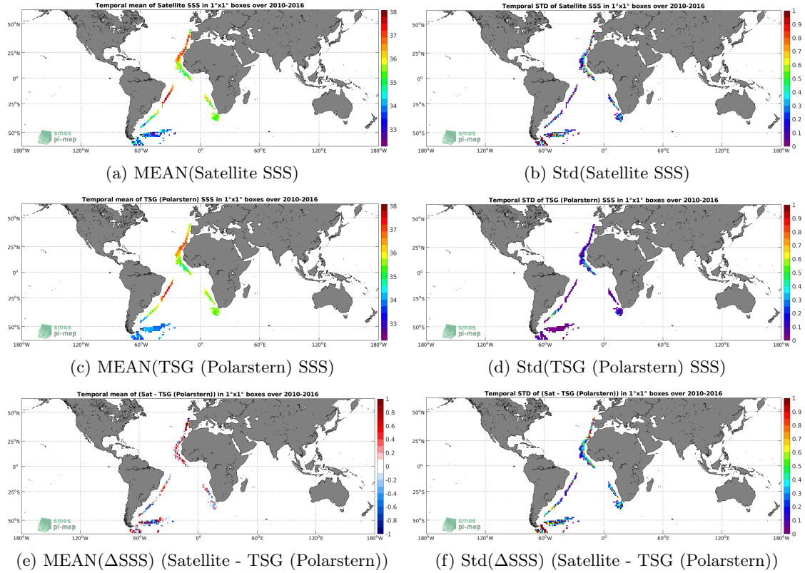
Figure 6: Temporal mean (left) and Std (right) of SSS from SMOS SSS L3 v3 Monthly (ICDC) (top), TSG (Polarstern) (middle), and of \Delta SSS (Satellite - TSG (Polarstern)). Only match-up pairs are used to generate these maps.
