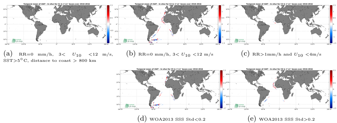
Figure 12: Temporal mean gridded over spatial boxes of size 1^\circ \times 1^\circ of \Delta SSS (SMOS SSS L3 v3 Monthly (ICDC) - TSG (Polarstern)) for 5 different subdatasets corresponding to:RR=0 mm/h, 3 < U_{10} < 12 m/s, SST >5^\circ C, distance to coast > 800 km (a), RR=0 mm/h, 3 < U_{10} < 12 m/s (b), RR >1 mm/h and U_{10} < 4 m/s (c), WOA2013 SSS Std <0.2 (d), WOA2013 SSS Std >0.2 (e).
