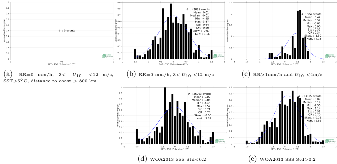
Figure 13: Normalized histogram of \Delta\text{SSS} (SMOS SSS L3 v3 Monthly (ICDC) - TSG (Polarstern)) for 5 different subdatasets corresponding to: RR=0 mm/h, 3 < U_{10} < 12 m/s, SST > 5^{\circ}\text{C} , distance to coast > 800 km (a), RR=0 mm/h, 3 < U_{10} < 12 m/s (b), RR > 1\text{mm/h} and U_{10} < 4\text{m/s} (c), WOA2013 SSS Std < 0.2 (d), WOA2013 SSS Std > 0.2 (e).
