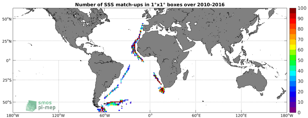
Figure 4: Number of SSS match-ups between TSG (Polarstern) SSS and the SMOS SSS L3 v3 Monthly (ICDC) SSS product for the SMOS coastal zone (<800km) 60N-60S Pi-MEP region over 1°x1° boxes and for the full satellite product period.
