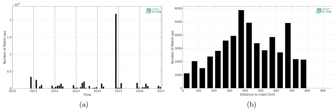
Figure 1: Number of match-ups between TSG-POLARSTERN and SMOS-L3-ICDC-V3-MONTHLY-0.5DEG SSS as a function of time (a) and as function of the distance to coast (b) over the SMOS coastal zone (<800km) 60N-60S Pi-MEP region and for the full satellite product period.
