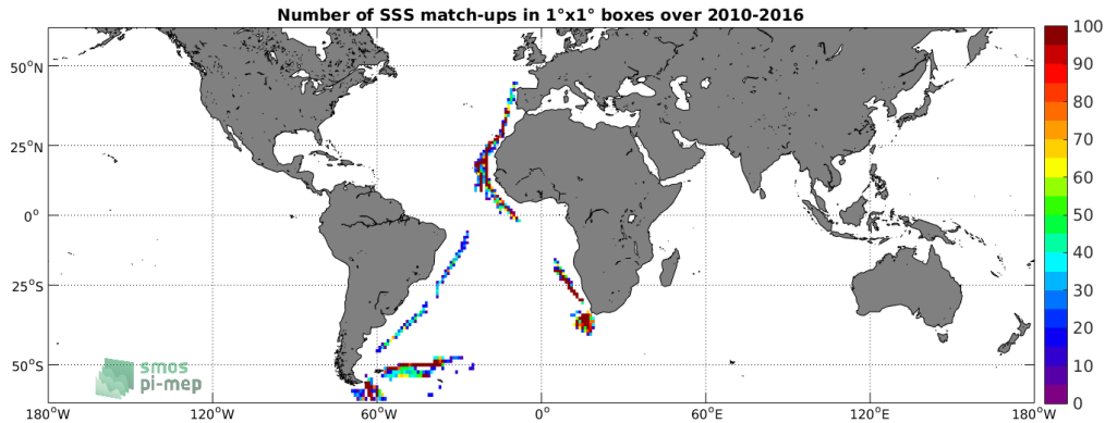
Figure 4: Number of SSS match-ups between TSG-POLARSTERN SSS and the SMOS-L3-ICDC-V3-MONTHLY-0.5DEG SSS product for the SMOS coastal zone (<800km) 60N-60S Pi-MEP region over 1°x1° boxes and for the full satellite product period.
