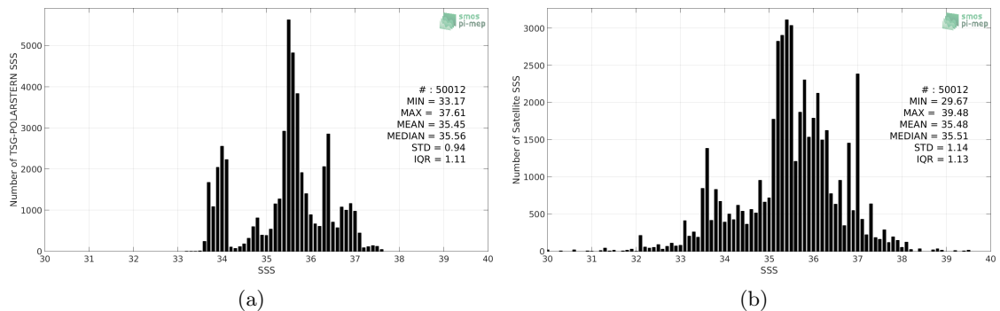
Figure 2: Histograms of SSS from TSG-POLARSTERN (a) and SMOS-L3-ICDC-V3-MONTHLY-0.5DEG (b) considering all match-up pairs per bins of 0.1 over the SMOS coastal zone (<800km) 60N-60S Pi-MEP region and for the full satellite product period.
