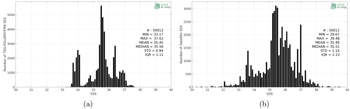
Figure 2: Histograms of SSS from TSG-POLARSTERN (a) and SMOS-L3-ICDC-V3-MONTHLY-0.5DEG (b) considering all match-up pairs per bins of 0.1 over the SMOS coastal zone ( \geq 800\text{km} ) 60N-60S Pi-MEP region and for the full satellite product period.
