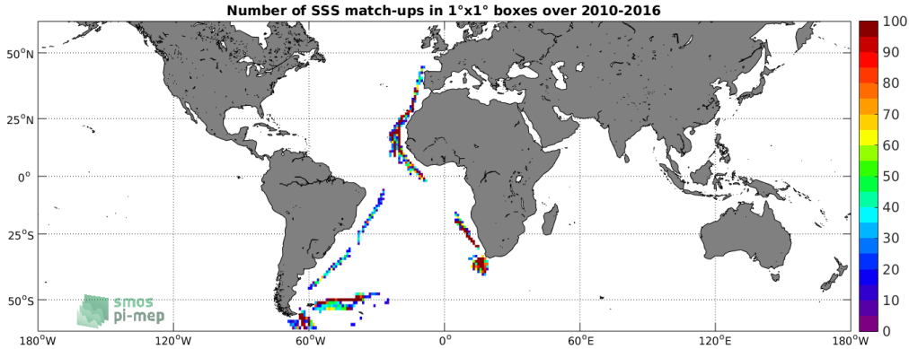
Figure 4: Number of SSS match-ups between TSG-POLARSTERN SSS and the SMOS-L3-ICDC-V3-MONTHLY-0.5DEG SSS product for the SMOS coastal zone ( \approx 800\text{km} ) 60N-60S Pi-MEP region over 1^\circ \times 1^\circ boxes and for the full satellite product period.
