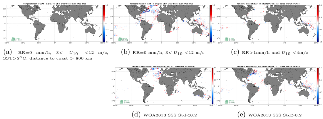
Figure 12: Temporal mean gridded over spatial boxes of size 1°x1° of \Delta SSS (SMOS SSS L3 v3 Monthly (ICDC) - TSG (LEGOS-DM)) for 5 different subdatasets corresponding to:RR=0 mm/h, 3 < U_{10} < 12 m/s, SST>5°C, distance to coast > 800 km (a), RR=0 mm/h, 3 < U_{10} < 12 m/s (b), RR>1mm/h and U_{10} < 4 m/s (c), WOA2013 SSS Std<0.2 (d), WOA2013 SSS Std>0.2 (e).
