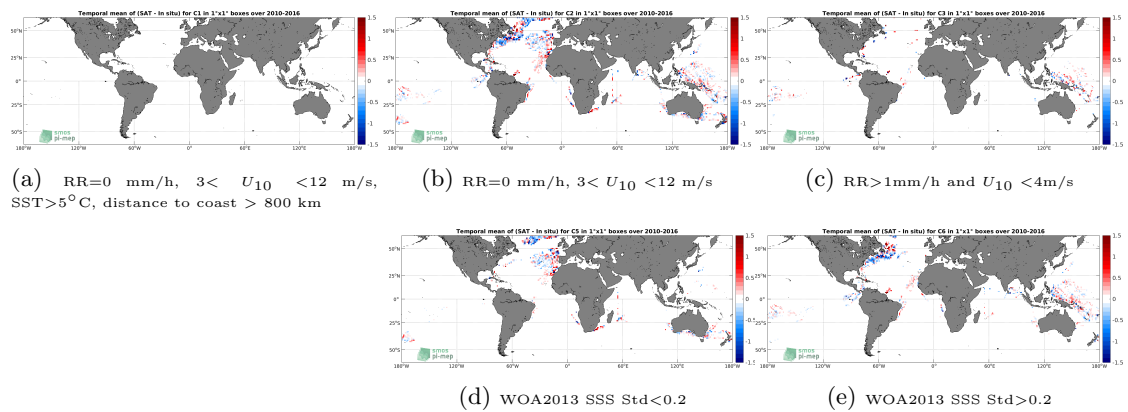
Figure 12: Temporal mean gridded over spatial boxes of size 1^\circ \times 1^\circ of \Delta SSS (SMOS SSS L3 v3 Monthly (ICDC) - TSG (LEGOS-DM)) for 5 different subdatasets corresponding to: RR=0 mm/h, 3 < U_{10} < 12 m/s, SST > 5^\circ\text{C} , distance to coast > 800 km (a), RR=0 mm/h, 3 < U_{10} < 12 m/s (b), RR > 1 mm/h and U_{10} < 4 m/s (c), WOA2013 SSS Std < 0.2 (d), WOA2013 SSS Std > 0.2 (e).
