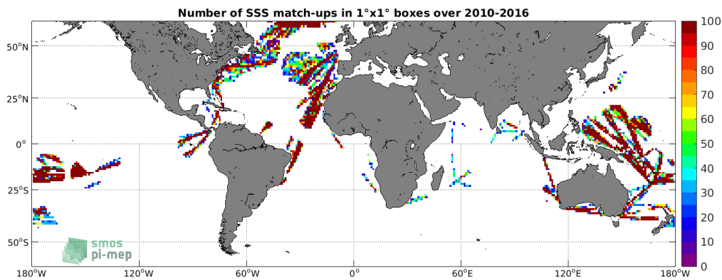
Figure 4: Number of SSS match-ups between TSG (LEGOS-DM) SSS and the SMOS SSS L3 v3 Monthly (ICDC) SSS product for the SMOS coastal zone (<800km) 60N-60S Pi-MEP region over 1°x1° boxes and for the full satellite product period.
