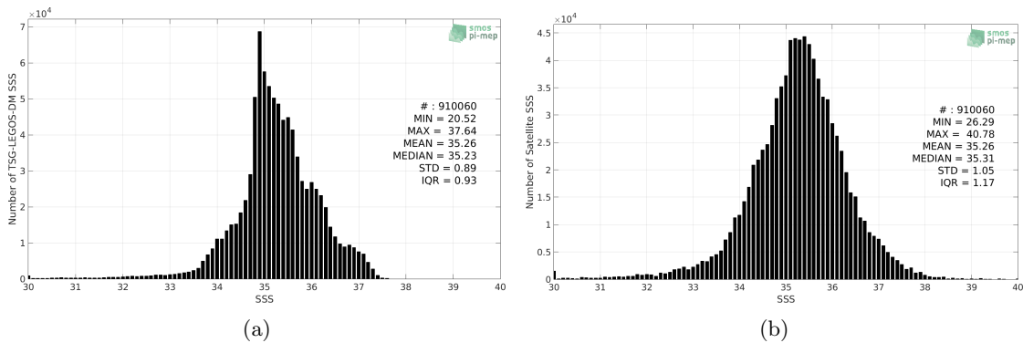
Figure 2: Histograms of SSS from TSG-LEGOS-DM (a) and SMOS-L3-ICDC-V3-MONTHLY-0.5DEG (b) considering all match-up pairs per bins of 0.1 over the SMOS coastal zone ( \approx 800\text{km} ) 60N-60S Pi-MEP region and for the full satellite product period.
