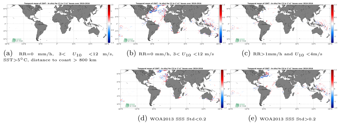
Figure 12: Temporal mean gridded over spatial boxes of size 1^\circ \times 1^\circ of \Delta SSS (SMOS-L3-ICDC-V3-MONTHLY-0.5DEG - TSG-LEGOS-DM) for 5 different subdatasets corresponding to:RR=0 mm/h, 3 < U_{10} < 12 m/s, SST >5^\circ C, distance to coast > 800 km (a), RR=0 mm/h, 3 < U_{10} < 12 m/s (b), RR >1 mm/h and U_{10} < 4 m/s (c), WOA2013 SSS Std <0.2 (d), WOA2013 SSS Std >0.2 (e).
