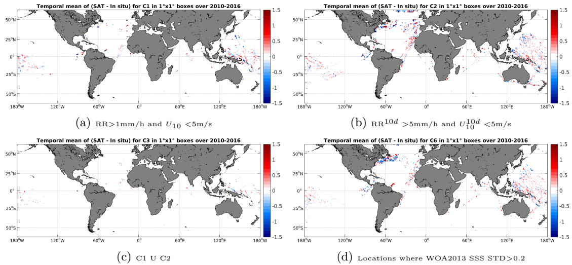
Figure 12: Temporal mean gridded over spatial boxes of size 1^\circ \times 1^\circ of \Delta SSS (SMOS-L3-ICDC-V3-MONTHLY-0.5DEG - TSG-LEGOS-DM) for 4 different subdatasets corresponding to: RR > 1\text{mm/h} and U_{10} < 5\text{m/s} (a), RR^{10d} > 5\text{mm/h} and U_{10}^{10d} < 5\text{m/s} (b), C1 U C2 (c), Locations where WOA2013 SSS STD > 0.2 (d).
