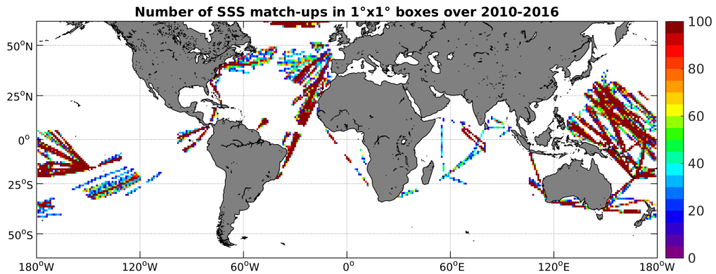
Figure 4: Number of SSS match-ups between TSG-LEGOS-DM SSS and the SMOS-L3-ICDC-V3-MONTHLY-0.5DEG SSS product for the SMOS coastal zone ( \pm 800\text{km} ) 60N-60S Pi-MEP region over 1^\circ \times 1^\circ boxes and for the full satellite product period.
