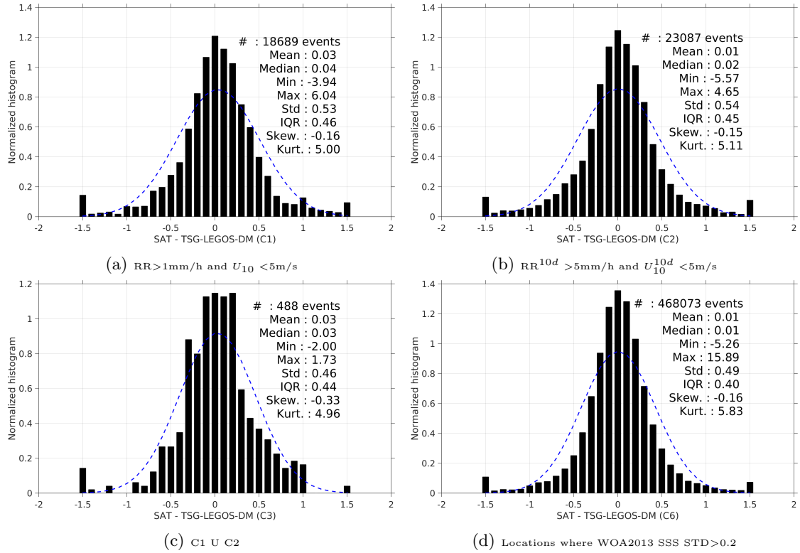
Figure 13: Normalized histogram of \Delta\text{SSS} (SMOS-L3-ICDC-V3-MONTHLY-0.5DEG - TSG-LEGOS-DM) for 6 different subdatasets corresponding to: \text{RR} > 1\text{mm/h} and U_{10} < 5\text{m/s} (a), \text{RR}^{10d} > 5\text{mm/h} and U_{10}^{10d} < 5\text{m/s} (b), C1 U C2 (c), Locations where WOA2013 SSS STD > 0.2 (d).
