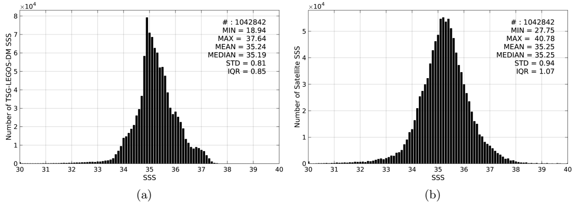
Figure 2: Histograms of SSS from TSG-LEGOS-DM (a) and SMOS-L3-ICDC-V3-MONTHLY-0.5DEG (b) considering all match-up pairs per bins of 0.1 over the SMOS coastal zone ( \approx 800 km) 60N-60S Pi-MEP region and for the full satellite product period.
