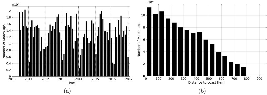
Figure 1: Number of match-ups between TSG-LEGOS-DM and SMOS-L3-ICDC-V3-MONTHLY-0.5DEG SSS as a function of time (a) and as function of the distance to coast (b) over the SMOS coastal zone ( \approx 800 km) 60N-60S Pi-MEP region and for the full satellite product period.
