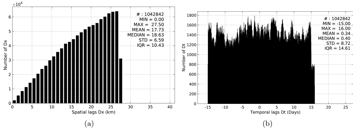
Figure 5: Histograms of the spatial (a) and temporal (b) lags between the time of the TSG-LEGOS-DM measurements and the date of the corresponding SMOS-L3-ICDC-V3-MONTHLY-0.5DEG SSS product.
