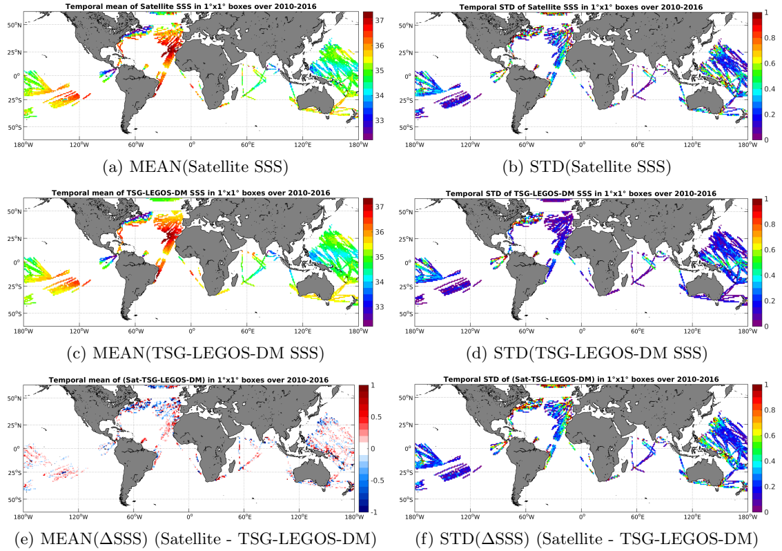
Figure 6: Temporal mean (left) and STD (right) of SSS from SMOS-L3-ICDC-V3-MONTHLY-0.5DEG (top), TSG-LEGOS-DM (middle), and of \Delta SSS (Satellite - TSG-LEGOS-DM). Only match-up pairs are used to generate these maps.
