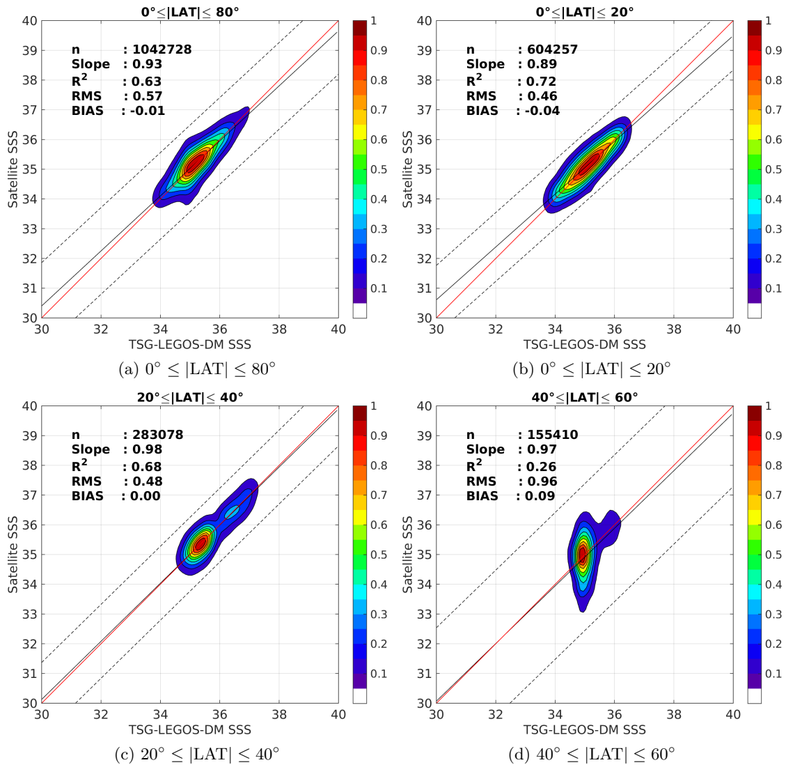
Figure 9: Contour maps of the concentration of SMOS-L3-ICDC-V3-MONTHLY-0.5DEG SSS (y-axis) versus TSG-LEGOS-DM SSS (x-axis) at match-up pairs for different latitude bands. For each plot, the red line shows x=y . The black thin and dashed lines indicate a linear fit through the data cloud and the \pm 95\% confidence levels, respectively. The number match-up pairs n , the slope and R^2 coefficient of the linear fit, the root mean square (RMS) and the mean bias between satellite and in situ data are indicated for each latitude band in each plots.
