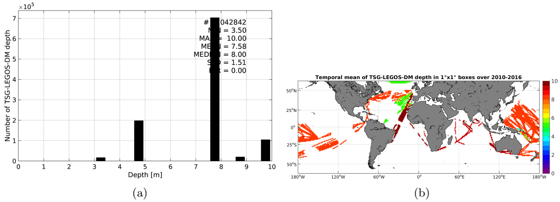
Figure 3: Histograms of the depth of the upper level SSS measurements from TSG-LEGOS-DM in the Match-up DataBase for the SMOS coastal zone ( \pm 800\text{km} ) 60N-60S Pi-MEP region (a) and temporal mean spatial distribution of pressure of the in situ SSS data over 1^\circ \times 1^\circ boxes and for the full satellite product period (b).
