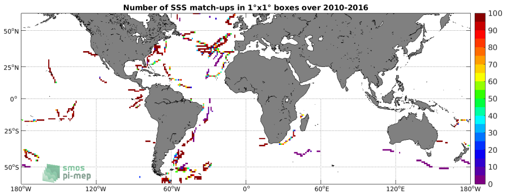
Figure 4: Number of SSS match-ups between TSG (GOSUD-Sailing-ship) SSS and the SMOS SSS L3 v3 Monthly (ICDC) SSS product for the SMOS coastal zone (<800km) 60N-60S Pi-MEP region over 1°x1° boxes and for the full satellite product period.
