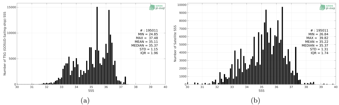
Figure 2: Histograms of SSS from TSG (GOSUD-Sailing-ship) (a) and SMOS SSS L3 v3 Monthly (ICDC) (b) considering all match-up pairs per bins of 0.1 over the SMOS coastal zone (<800km) 60N-60S Pi-MEP region and for the full satellite product period.
