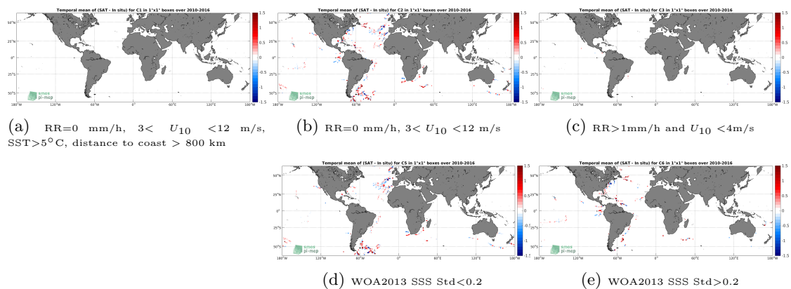
Figure 12: Temporal mean gridded over spatial boxes of size 1^\circ \times 1^\circ of \Delta\text{SSS} (SMOS-L3-ICDC-V3-MONTHLY-0.5DEG - TSG-GOSUD-Sailing-ship) for 5 different subdatasets corresponding to: RR=0 mm/h, 3 < U_{10} < 12 m/s, SST > 5°C, distance to coast > 800 km (a), RR=0 mm/h, 3 < U_{10} < 12 m/s (b), RR > 1mm/h and U_{10} < 4 m/s (c), WOA2013 SSS Std < 0.2 (d), WOA2013 SSS Std > 0.2 (e).
