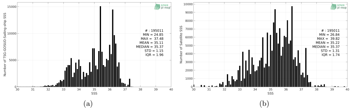
Figure 2: Histograms of SSS from TSG-GOSUD-Sailing-ship (a) and SMOS-L3-ICDC-V3-MONTHLY-0.5DEG (b) considering all match-up pairs per bins of 0.1 over the SMOS coastal zone (<800km) 60N-60S Pi-MEP region and for the full satellite product period.
