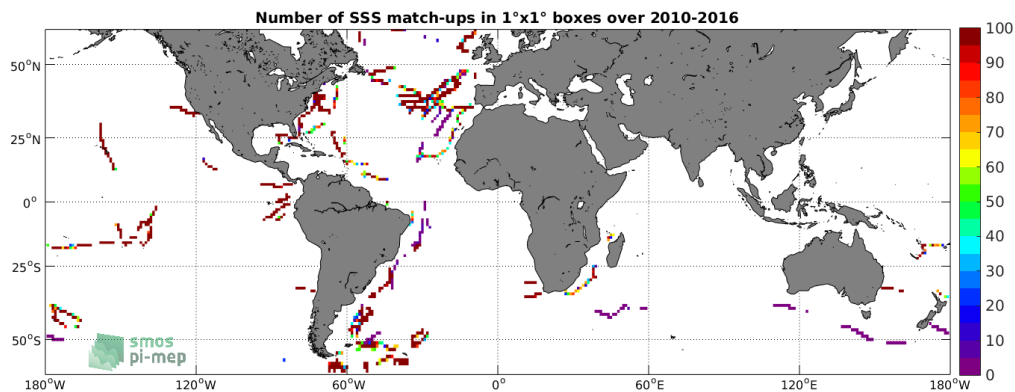
Figure 4: Number of SSS match-ups between TSG-GOSUD-Sailing-ship SSS and the SMOS-L3-ICDC-V3-MONTHLY-0.5DEG SSS product for the SMOS coastal zone (<800km) 60N-60S Pi-MEP region over 1°x1° boxes and for the full satellite product period.
