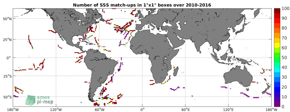
Figure 4: Number of SSS match-ups between TSG-GOSUD-Sailing-ship SSS and the SMOS-L3-ICDC-V3-MONTHLY-0.5DEG SSS product for the SMOS coastal zone ( \pm 800\text{km} ) 60N-60S Pi-MEP region over 1^\circ \times 1^\circ boxes and for the full satellite product period.
