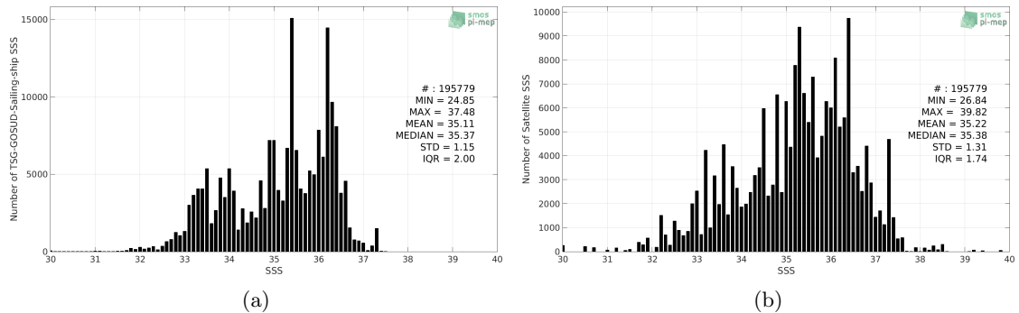
Figure 2: Histograms of SSS from TSG-GOSUD-Sailing-ship (a) and SMOS-L3-ICDC-V3-MONTHLY-0.5DEG (b) considering all match-up pairs per bins of 0.1 over the SMOS coastal zone ( \approx 800 km) 60N-60S Pi-MEP region and for the full satellite product period.
