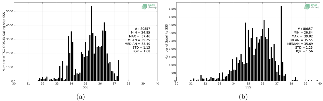
Figure 2: Histograms of SSS from TSG-GOSUD-Sailing-ship (a) and SMOS-L3-ICDC-V3-MONTHLY-0.5DEG (b) considering all match-up pairs per bins of 0.1 over the SMOS coastal zone ( \approx 800\text{km} ) 60N-60S Pi-MEP region and for the full satellite product period.
