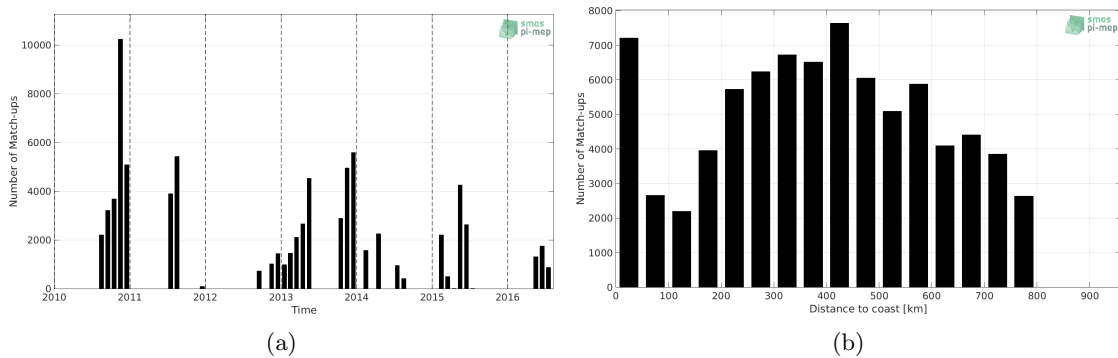
Figure 1: Number of match-ups between TSG-GOSUD-Sailing-ship and SMOS-L3-ICDC-V3-MONTHLY-0.5DEG SSS as a function of time (a) and as function of the distance to coast (b) over the SMOS coastal zone ( \approx 800\text{km} ) 60N-60S Pi-MEP region and for the full satellite product period.
