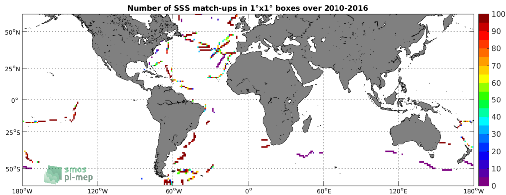
Figure 4: Number of SSS match-ups between TSG-GOSUD-Sailing-ship SSS and the SMOS-L3-ICDC-V3-MONTHLY-0.5DEG SSS product for the SMOS coastal zone ( \approx 800\text{km} ) 60N-60S Pi-MEP region over 1^\circ \times 1^\circ boxes and for the full satellite product period.
