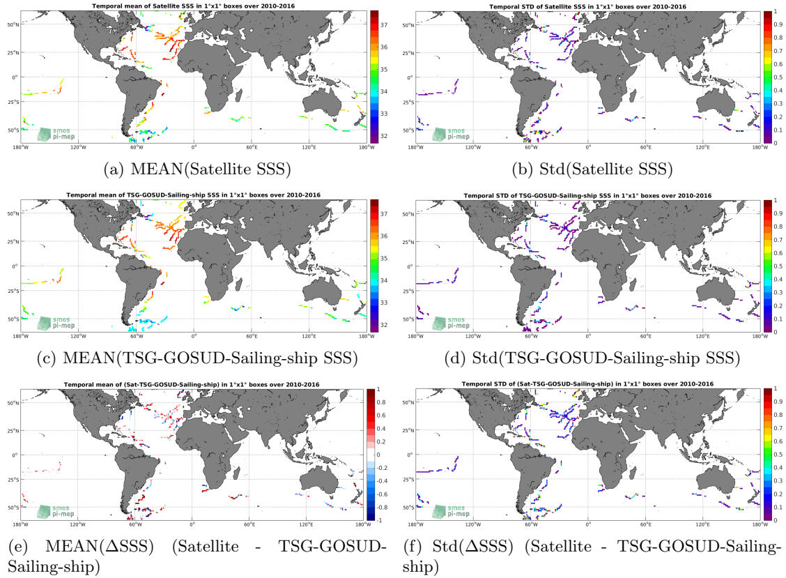
Figure 6: Temporal mean (left) and Std (right) of SSS from SMOS-L3-ICDC-V3-MONTHLY-0.5DEG (top), TSG-GOSUD-Sailing-ship (middle), and of \Delta SSS (Satellite - TSG-GOSUD-Sailing-ship). Only match-up pairs are used to generate these maps.
