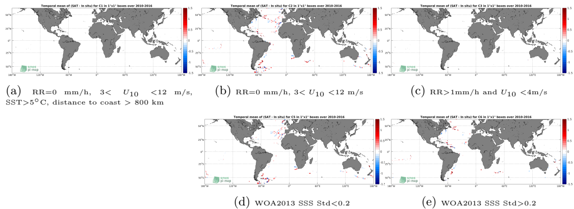
Figure 12: Temporal mean gridded over spatial boxes of size 1^\circ \times 1^\circ of \Delta SSS (SMOS-L3-ICDC-V3-MONTHLY-0.5DEG - TSG-GOSUD-Sailing-ship) for 5 different subdatasets corresponding to:RR=0 mm/h, 3 < U_{10} < 12 m/s, SST >5^\circ C, distance to coast > 800 km (a), RR=0 mm/h, 3 < U_{10} < 12 m/s (b), RR >1 mm/h and U_{10} < 4 m/s (c), WOA2013 SSS Std <0.2 (d), WOA2013 SSS Std >0.2 (e).
