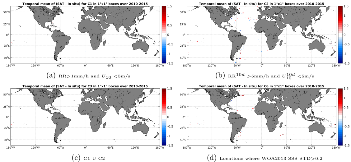
Figure 12: Temporal mean gridded over spatial boxes of size 1^\circ \times 1^\circ of \Delta SSS (SMOS-L3-ICDC-V3-MONTHLY-0.5DEG - TSG-GOSUD-Sailing-ship) for 4 different subdatasets corresponding to: RR > 1 mm/h and U_{10} < 5 m/s (a), RR 10d > 5 mm/h and U_{10}^{10d} < 5 m/s (b), C1 U C2 (c), Locations where WOA2013 SSS STD > 0.2 (d).
