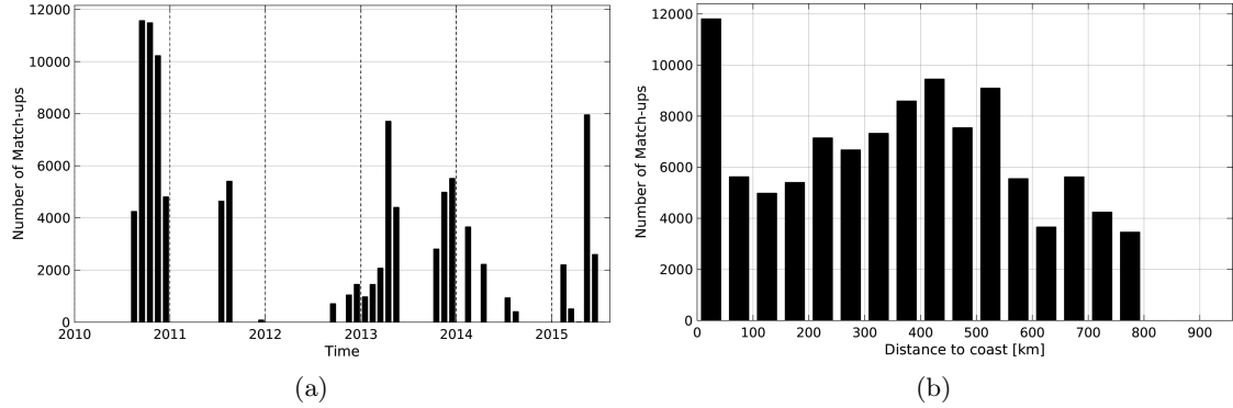
Figure 1: Number of match-ups between TSG-GOSUD-Sailing-ship and SMOS-L3-ICDC-V3-MONTHLY-0.5DEG SSS as a function of time (a) and as function of the distance to coast (b) over the SMOS coastal zone ( \approx 800\text{km} ) 60N-60S Pi-MEP region and for the full satellite product period.
