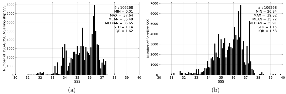
Figure 2: Histograms of SSS from TSG-GOSUD-Sailing-ship (a) and SMOS-L3-ICDC-V3-MONTHLY-0.5DEG (b) considering all match-up pairs per bins of 0.1 over the SMOS coastal zone ( \approx 800\text{km} ) 60N-60S Pi-MEP region and for the full satellite product period.
