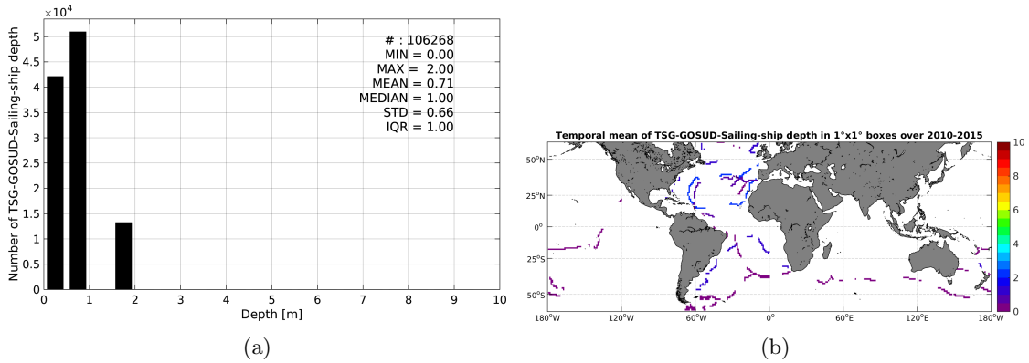
Figure 3: Histograms of the depth of the upper level SSS measurements from TSG-GOSUD-Sailing-ship in the Match-up DataBase for the SMOS coastal zone ( \approx 800 km) 60N-60S Pi-MEP region (a) and temporal mean spatial distribution of pressure of the in situ SSS data over 1^\circ \times 1^\circ boxes and for the full satellite product period (b).
