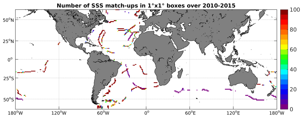
Figure 4: Number of SSS match-ups between TSG-GOSUD-Sailing-ship SSS and the SMOS-L3-ICDC-V3-MONTHLY-0.5DEG SSS product for the SMOS coastal zone ( \approx 800 km) 60N-60S Pi-MEP region over 1^\circ \times 1^\circ boxes and for the full satellite product period.
