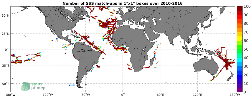
Figure 4: Number of SSS match-ups between TSG (GOSUD-Research-vessel) SSS and the SMOS SSS L3 v3 Monthly (ICDC) SSS product for the SMOS coastal zone ( <800\text{km} ) 60N-60S Pi-MEP region over 1^\circ \times 1^\circ boxes and for the full satellite product period.
