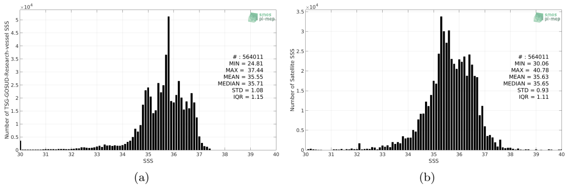
Figure 2: Histograms of SSS from TSG-GOSUD-Research-vessel (a) and SMOS-L3-ICDC-V3-MONTHLY-0.5DEG (b) considering all match-up pairs per bins of 0.1 over the SMOS coastal zone (<800km) 60N-60S Pi-MEP region and for the full satellite product period.
