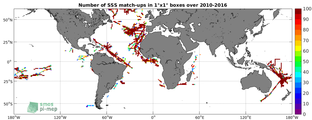
Figure 4: Number of SSS match-ups between TSG-GOSUD-Research-vessel SSS and the SMOS-L3-ICDC-V3-MONTHLY-0.5DEG SSS product for the SMOS coastal zone (<800km) 60N-60S Pi-MEP region over 1^\circ \times 1^\circ boxes and for the full satellite product period.
