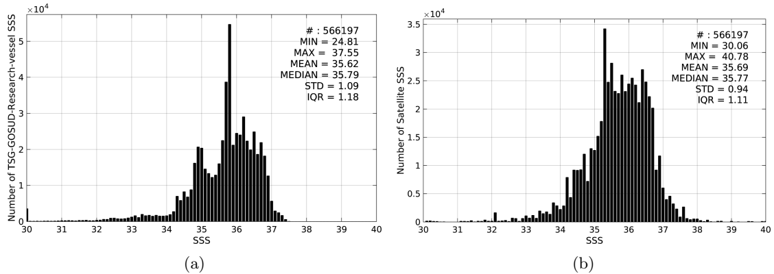
Figure 2: Histograms of SSS from TSG-GOSUD-Research-vessel (a) and SMOS-L3-ICDC-V3-MONTHLY-0.5DEG (b) considering all match-up pairs per bins of 0.1 over the SMOS coastal zone ( \approx 800 km) 60N-60S Pi-MEP region and for the full satellite product period.
