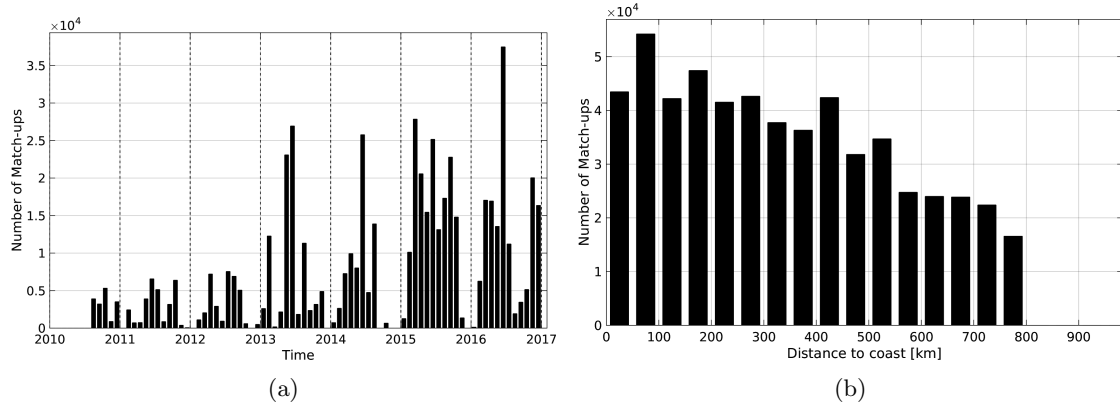
Figure 1: Number of match-ups between TSG-GOSUD-Research-vessel and SMOS-L3-ICDC-V3-MONTHLY-0.5DEG SSS as a function of time (a) and as function of the distance to coast (b) over the SMOS coastal zone ( \approx 800 km) 60N-60S Pi-MEP region and for the full satellite product period.
