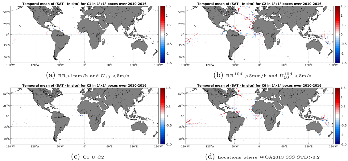
Figure 12: Temporal mean gridded over spatial boxes of size 1^\circ \times 1^\circ of \Delta SSS (SMOS-L3-ICDC-V3-MONTHLY-0.5DEG - TSG-GOSUD-Research-vessel) for 4 different subdatasets corresponding to: RR > 1\text{mm/h} and U_{10} < 5\text{m/s} (a), RR^{10d} > 5\text{mm/h} and U_{10}^{10d} < 5\text{m/s} (b), C1 U C2 (c), Locations where WOA2013 SSS STD > 0.2 (d).
