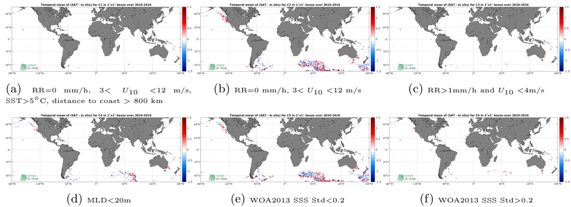
Figure 12: Temporal mean gridded over spatial boxes of size 1^\circ \times 1^\circ of \Delta SSS (SMOS SSS L3 v3 Monthly (ICDC) - Marine mammals) for 6 different subdatasets corresponding to:RR=0 mm/h, 3 < U_{10} < 12 m/s, SST >5^\circ C, distance to coast > 800 km (a), RR=0 mm/h, 3 < U_{10} < 12 m/s (b), RR >1 mm/h and U_{10} < 4 m/s (c),MLD <20 m (d),WOA2013 SSS Std <0.2 (e),WOA2013 SSS Std >0.2 (f).
