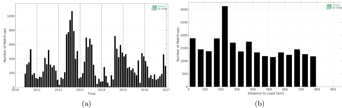
Figure 1: Number of match-ups between Marine mammals and SMOS SSS L3 v3 Monthly (ICDC) SSS as a function of time (a) and as function of the distance to coast (b) over the SMOS coastal zone (<800km) 60N-60S Pi-MEP region and for the full satellite product period.
