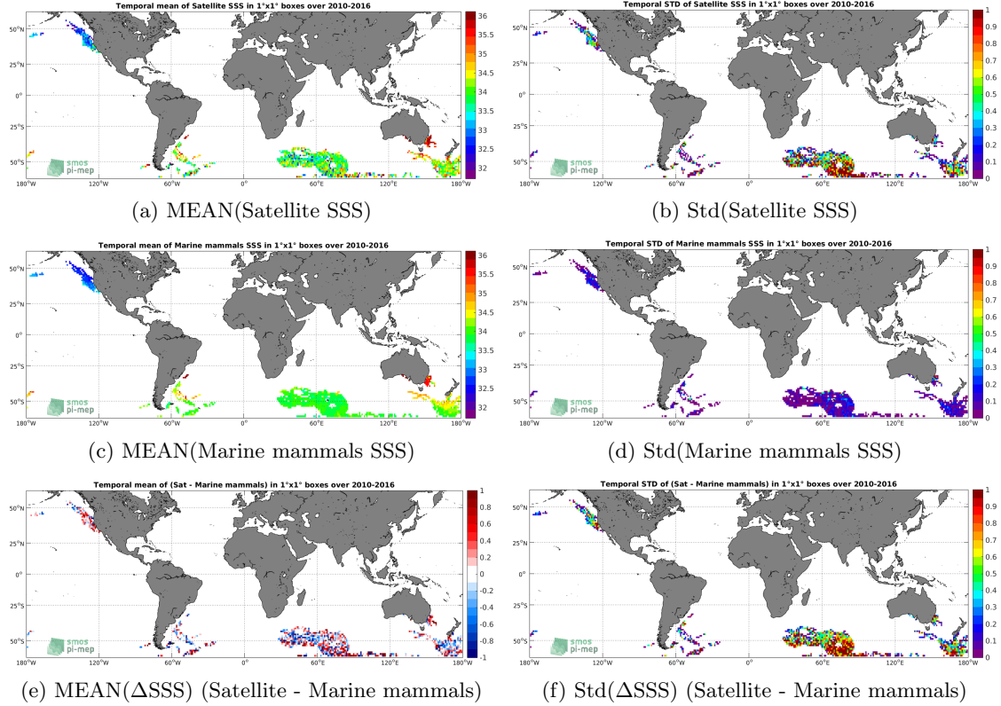
Figure 6: Temporal mean (left) and Std (right) of SSS from SMOS SSS L3 v3 Monthly (ICDC) (top), Marine mammals (middle), and of \Delta SSS (Satellite - Marine mammals). Only match-up pairs are used to generate these maps.
