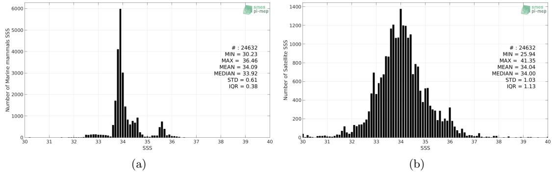
Figure 2: Histograms of SSS from Marine mammals (a) and SMOS SSS L3 v3 Monthly (ICDC) (b) considering all match-up pairs per bins of 0.1 over the SMOS coastal zone (<800km) 60N-60S Pi-MEP region and for the full satellite product period.
