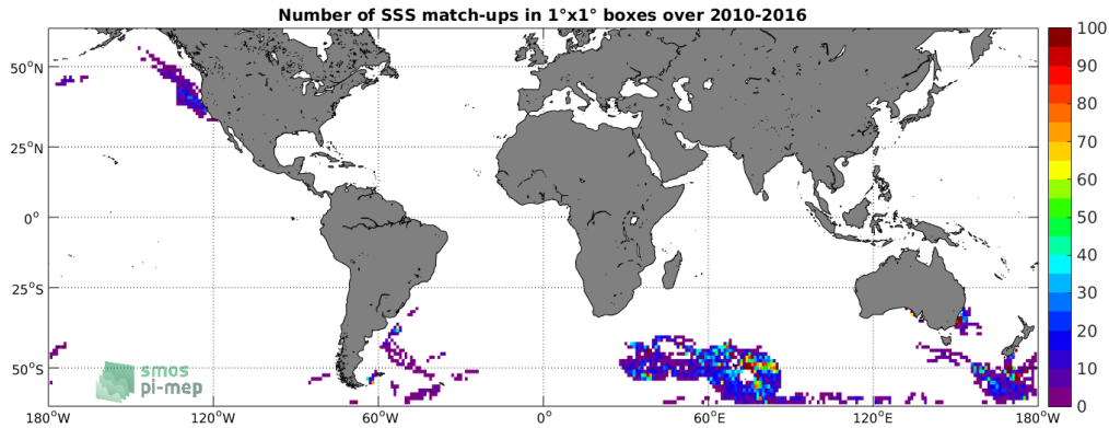
Figure 4: Number of SSS match-ups between Marine mammals SSS and the SMOS SSS L3 v3 Monthly (ICDC) SSS product for the SMOS coastal zone (<800km) 60N-60S Pi-MEP region over 1^\circ \times 1^\circ boxes and for the full satellite product period.
