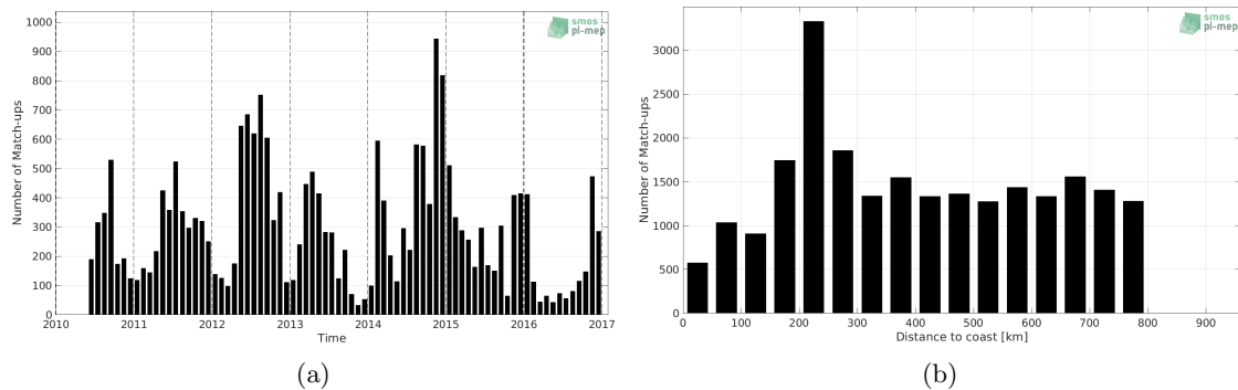
Figure 1: Number of match-ups between Sea mammals and SMOS SSS L3 v3 Monthly (ICDC) SSS as a function of time (a) and as function of the distance to coast (b) over the SMOS coastal zone (<800km) 60N-60S Pi-MEP region and for the full satellite product period.
