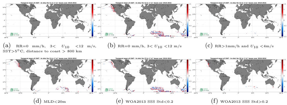
Figure 12: Temporal mean gridded over spatial boxes of size 1°x1° of \Delta SSS (SMOS SSS L3 v3 Monthly (ICDC) - Sea mammals) for 6 different subdatasets corresponding to:RR=0 mm/h, 3 < U_{10} < 12 m/s, SST > 5°C, distance to coast > 800 km (a), RR=0 mm/h, 3 < U_{10} < 12 m/s (b), RR > 1mm/h and U_{10} < 4 m/s (c),MLD < 20m (d),WOA2013 SSS Std < 0.2 (e),WOA2013 SSS Std > 0.2 (f).
