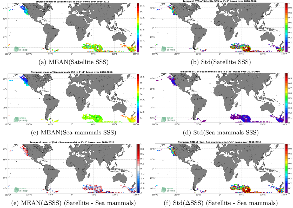
Figure 6: Temporal mean (left) and Std (right) of SSS from SMOS SSS L3 v3 Monthly (ICDC) (top), Sea mammals (middle), and of \Delta SSS (Satellite - Sea mammals). Only match-up pairs are used to generate these maps.
