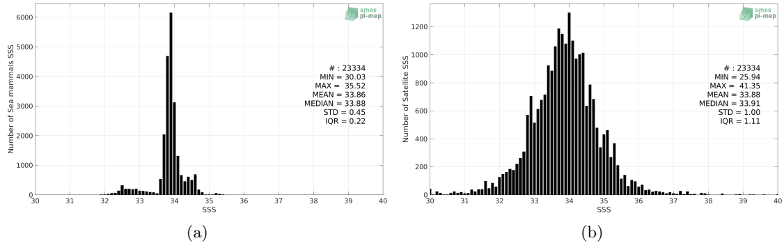
Figure 2: Histograms of SSS from Sea mammals (a) and SMOS SSS L3 v3 Monthly (ICDC) (b) considering all match-up pairs per bins of 0.1 over the SMOS coastal zone (<800km) 60N-60S Pi-MEP region and for the full satellite product period.
