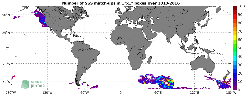
Figure 4: Number of SSS match-ups between Sea mammals SSS and the SMOS SSS L3 v3 Monthly (ICDC) SSS product for the SMOS coastal zone (<800km) 60N-60S Pi-MEP region over 1^\circ \times 1^\circ boxes and for the full satellite product period.
