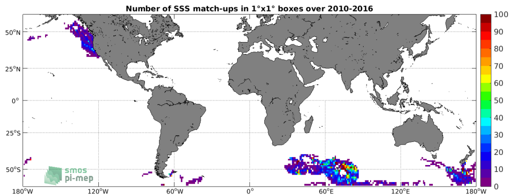
Figure 4: Number of SSS match-ups between Sea mammals SSS and the SMOS SSS L3 v3 Monthly (ICDC) SSS product for the SMOS coastal zone (<800km) 60N-60S Pi-MEP region over 1°x1° boxes and for the full satellite product period.
