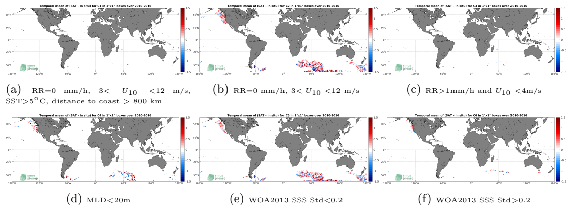
Figure 12: Temporal mean gridded over spatial boxes of size 1^\circ \times 1^\circ of \Delta SSS (SMOS SSS L3 v3 Monthly (ICDC) - Sea mammals) for 6 different subdatasets corresponding to:RR=0 mm/h, 3 < U_{10} < 12 m/s, SST >5^\circ C, distance to coast > 800 km (a), RR=0 mm/h, 3 < U_{10} < 12 m/s (b), RR >1 mm/h and U_{10} < 4 m/s (c),MLD <20 m (d),WOA2013 SSS Std <0.2 (e),WOA2013 SSS Std >0.2 (f).
