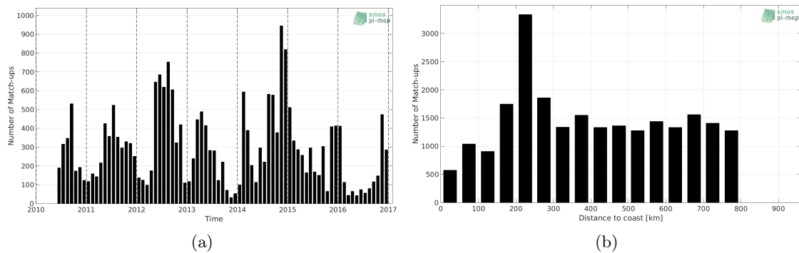
Figure 1: Number of match-ups between Sea mammals and SMOS-L3-ICDC-V3-MONTHLY-0.5DEG SSS as a function of time (a) and as function of the distance to coast (b) over the SMOS coastal zone (<800km) 60N-60S Pi-MEP region and for the full satellite product period.
