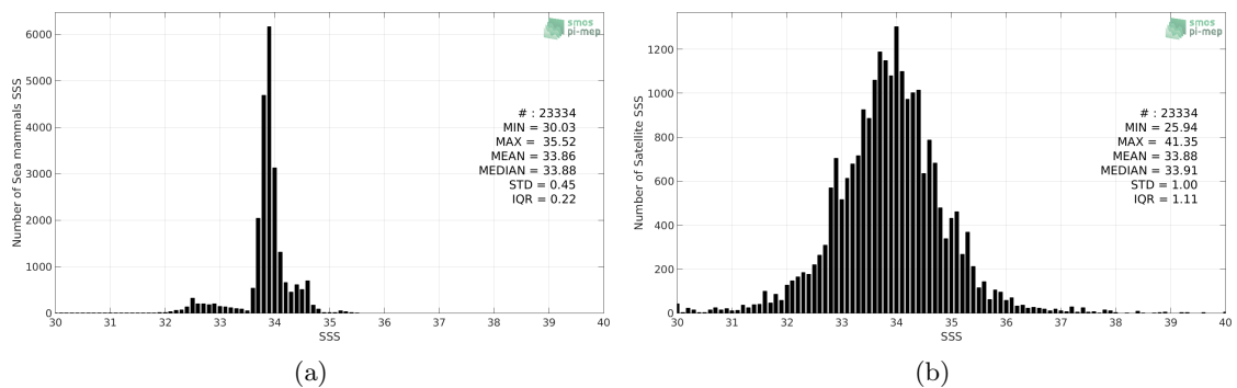
Figure 2: Histograms of SSS from Sea mammals (a) and SMOS-L3-ICDC-V3-MONTHLY-0.5DEG (b) considering all match-up pairs per bins of 0.1 over the SMOS coastal zone (<800km) 60N-60S Pi-MEP region and for the full satellite product period.
