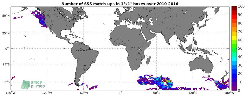
Figure 4: Number of SSS match-ups between Sea mammals SSS and the SMOS-L3-ICDC-V3-MONTHLY-0.5DEG SSS product for the SMOS coastal zone (<800km) 60N-60S Pi-MEP region over 1°x1° boxes and for the full satellite product period.
