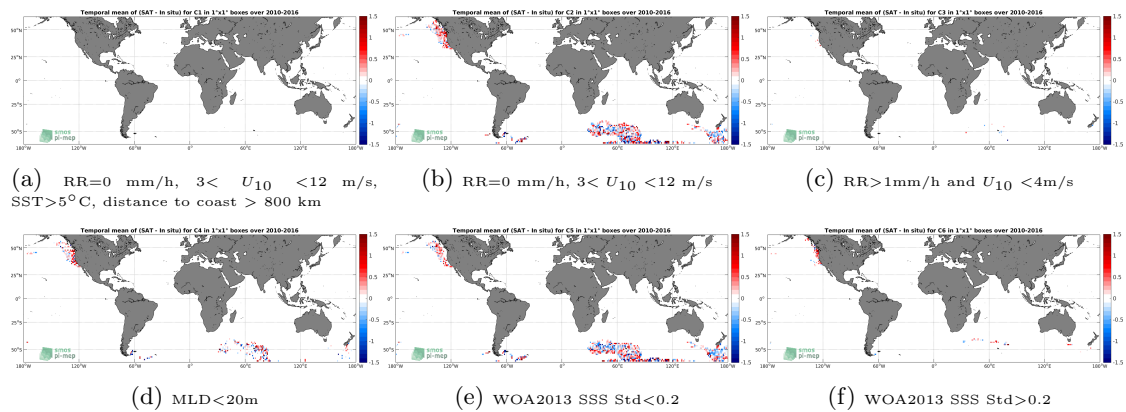
Figure 12: Temporal mean gridded over spatial boxes of size 1^\circ \times 1^\circ of \Delta SSS (SMOS-L3-ICDC-V3-MONTHLY-0.5DEG - Sea mammals) for 6 different subdatasets corresponding to:RR=0 mm/h, 3 < U_{10} < 12 m/s, SST >5^\circ C, distance to coast > 800 km (a), RR=0 mm/h, 3 < U_{10} < 12 m/s (b), RR >1 mm/h and U_{10} < 4 m/s (c),MLD <20 m (d),WOA2013 SSS Std <0.2 (e),WOA2013 SSS Std >0.2 (f).
