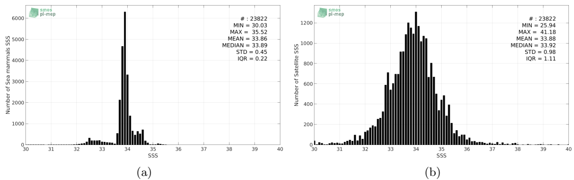
Figure 2: Histograms of SSS from Sea mammals (a) and SMOS-L3-ICDC-V3-MONTHLY-0.5DEG (b) considering all match-up pairs per bins of 0.1 over the SMOS coastal zone ( \approx 800\text{km} ) 60N-60S Pi-MEP region and for the full satellite product period.
