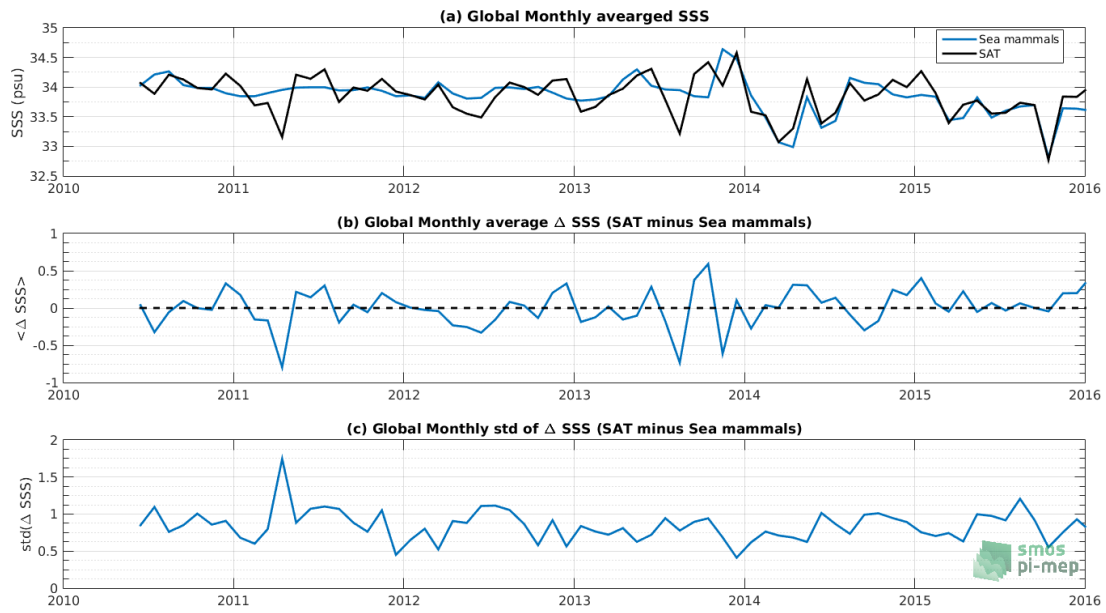
Figure 7: Time series of the monthly averaged mean SSS (top), mean \Delta SSS (Satellite - Sea mammals) and STD of \Delta SSS (Satellite - Sea mammals) over the SMOS coastal zone ( \pm 800\text{km} ) 60N-60S Pi-MEP region considering all match-ups collected by the Pi-MEP platform.
