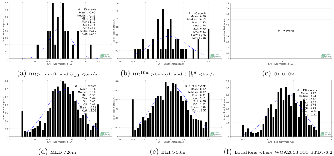
Figure 13: Normalized histogram of \Delta SSS (SMOS-L3-ICDC-V3-MONTHLY-0.5DEG - Sea mammals) for 6 different subdatasets corresponding to: RR > 1\text{mm/h} and U_{10} < 5\text{m/s} (a), RR^{10d} > 5\text{mm/h} and U_{10}^{10d} < 5\text{m/s} (b), C1 U C2 (c), MLD < 20\text{m} (d), BLT > 10\text{m} (e), Locations where WOA2013 SSS STD > 0.2 (f).
