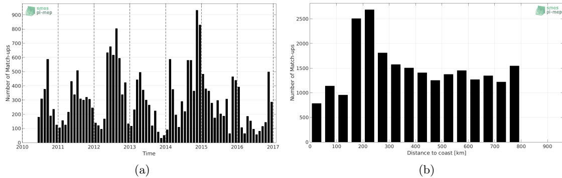
Figure 1: Number of match-ups between Sea mammals and SMOS-L3-ICDC-V3-MONTHLY-0.5DEG SSS as a function of time (a) and as function of the distance to coast (b) over the SMOS coastal zone ( \approx 800\text{km} ) 60N-60S Pi-MEP region and for the full satellite product period.
