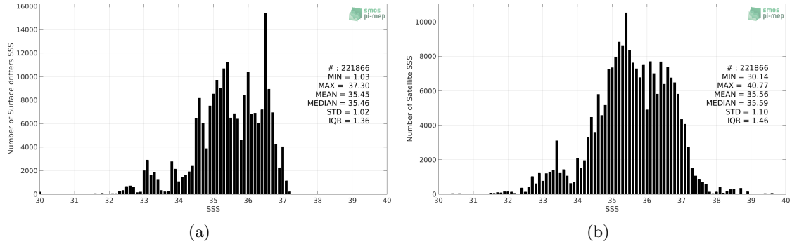
Figure 2: Histograms of SSS from Surface drifters (a) and SMOS SSS L3 v3 Monthly (ICDC) (b) considering all match-up pairs per bins of 0.1 over the SMOS coastal zone (<800km) 60N-60S Pi-MEP region and for the full satellite product period.
