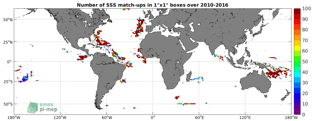
Figure 3: Number of SSS match-ups between Surface drifters SSS and the SMOS SSS L3 v3 Monthly (ICDC) SSS product for the SMOS coastal zone (<800km) 60N-60S Pi-MEP region over 1°x1° boxes and for the full satellite product period.
