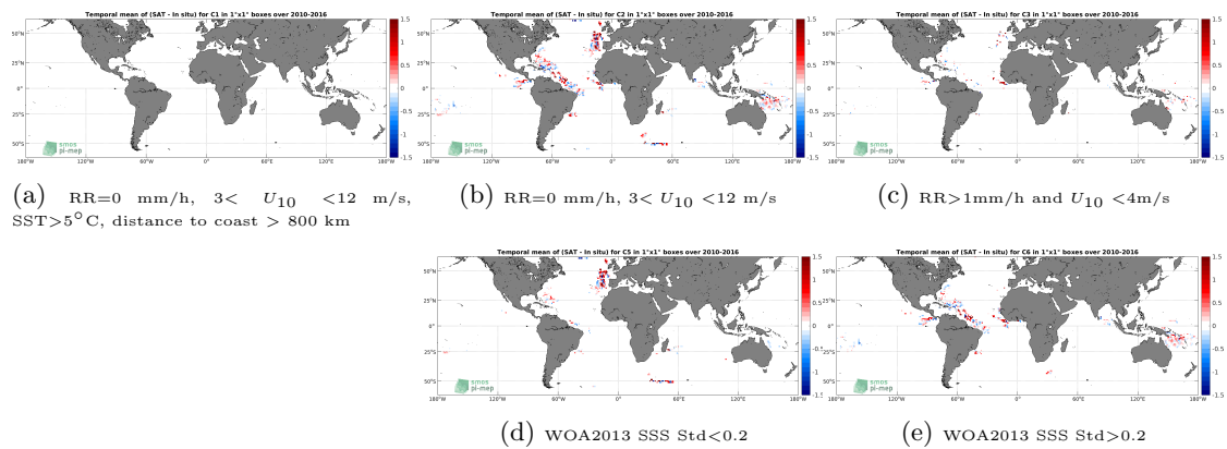
Figure 11: Temporal mean gridded over spatial boxes of size 1^\circ \times 1^\circ of \Delta\text{SSS} (SMOS SSS L3 v3 Monthly (ICDC) - Surface drifters) for 5 different subdatasets corresponding to: RR=0 mm/h, 3 < U_{10} < 12 m/s, SST > 5°C, distance to coast > 800 km (a), RR=0 mm/h, 3 < U_{10} < 12 m/s (b), RR > 1mm/h and U_{10} < 4 m/s (c), WOA2013 SSS Std < 0.2 (d), WOA2013 SSS Std > 0.2 (e).
