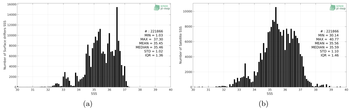
Figure 2: Histograms of SSS from Surface drifters (a) and SMOS-L3-ICDC-V3-MONTHLY-0.5DEG (b) considering all match-up pairs per bins of 0.1 over the SMOS coastal zone (<800km) 60N-60S Pi-MEP region and for the full satellite product period.
