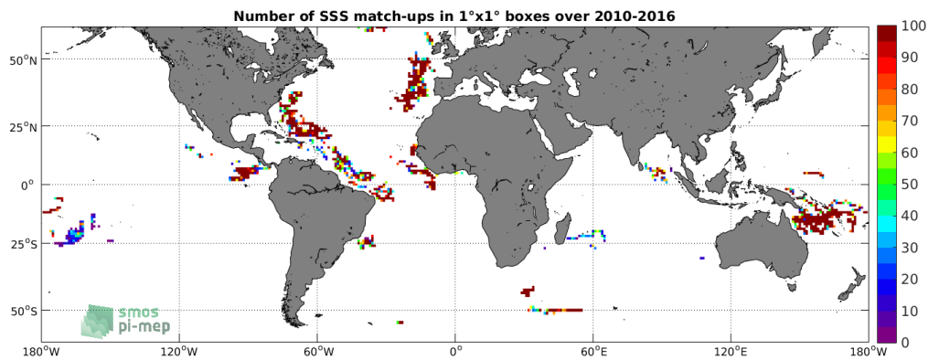
Figure 3: Number of SSS match-ups between Surface drifters SSS and the SMOS-L3-ICDC-V3-MONTHLY-0.5DEG SSS product for the SMOS coastal zone (<800km) 60N-60S Pi-MEP region over 1°x1° boxes and for the full satellite product period.
