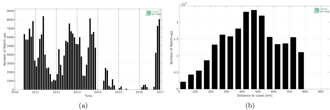
Figure 1: Number of match-ups between Surface drifters and SMOS-L3-ICDC-V3-MONTHLY-0.5DEG SSS as a function of time (a) and as function of the distance to coast (b) over the SMOS coastal zone (<800km) 60N-60S Pi-MEP region and for the full satellite product period.
