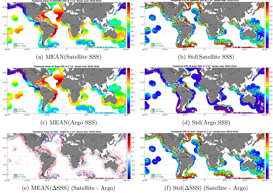
Figure 6: Temporal mean (left) and Std (right) of SSS from SMOS SSS L3 v3 Monthly (ICDC) (top), Argo (middle), and of \Delta SSS (Satellite - Argo). Only match-up pairs are used to generate these maps.
