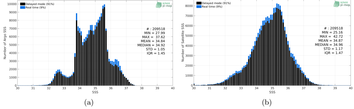
Figure 2: Histograms of SSS from Argo (a) and SMOS SSS L3 v3 Monthly (ICDC) (b) considering all match-up pairs per bins of 0.1 over the SMOS coastal zone (<800km) 60N-60S Pi-MEP region and for the full satellite product period.
