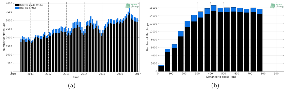
Figure 1: Number of match-ups between Argo and SMOS SSS L3 v3 Monthly (ICDC) SSS as a function of time (a) and as function of the distance to coast (b) over the SMOS coastal zone (<800km) 60N-60S Pi-MEP region and for the full satellite product period.
