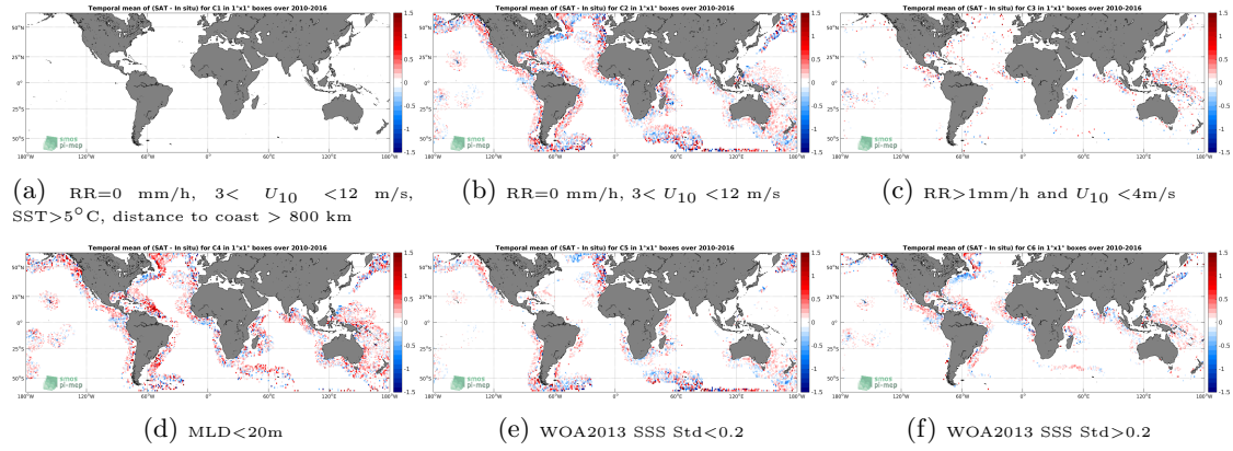
Figure 12: Temporal mean gridded over spatial boxes of size 1^\circ \times 1^\circ of \Delta SSS (SMOS SSS L3 v3 Monthly (ICDC) - Argo) for 6 different subdatasets corresponding to: RR=0 mm/h, 3 < U_{10} < 12 m/s, SST > 5^\circ\text{C} , distance to coast > 800 km (a), RR=0 mm/h, 3 < U_{10} < 12 m/s (b), RR > 1 mm/h and U_{10} < 4 m/s (c), MLD < 20 m (d), WOA2013 SSS Std < 0.2 (e), WOA2013 SSS Std > 0.2 (f).
