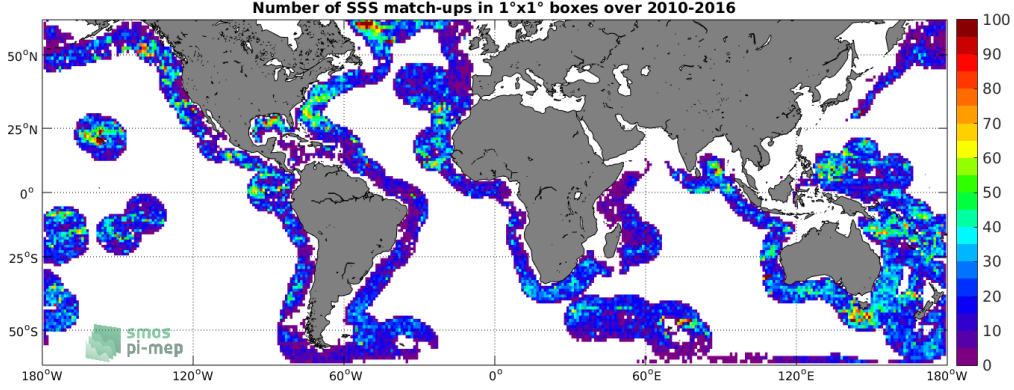
Figure 4: Number of SSS match-ups between Argo SSS and the SMOS SSS L3 v3 Monthly (ICDC) SSS product for the SMOS coastal zone (<800km) 60N-60S Pi-MEP region over 1^\circ \times 1^\circ boxes and for the full satellite product period.
