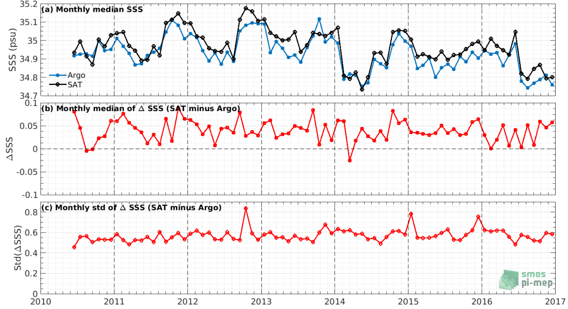
Figure 7: Time series of the monthly median SSS (top), median of \Delta SSS (Satellite - Argo) and Std of \Delta SSS (Satellite - Argo) over the SMOS coastal zone ( <800\text{km} ) 60\text{N} - 60\text{S} Pi-MEP region considering all match-ups collected by the Pi-MEP.
