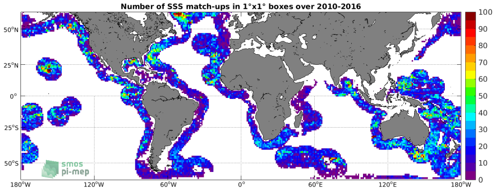
Figure 4: Number of SSS match-ups between Argo SSS and the SMOS SSS L3 v3 Monthly (ICDC) SSS product for the SMOS coastal zone (<800km) 60N-60S Pi-MEP region over 1°x1° boxes and for the full satellite product period.
