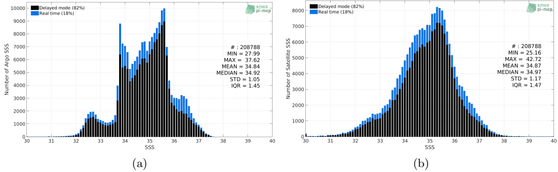
Figure 2: Histograms of SSS from Argo (a) and SMOS-L3-ICDC-V3-MONTHLY-0.5DEG (b) considering all match-up pairs per bins of 0.1 over the SMOS coastal zone (<800km) 60N-60S Pi-MEP region and for the full satellite product period.
