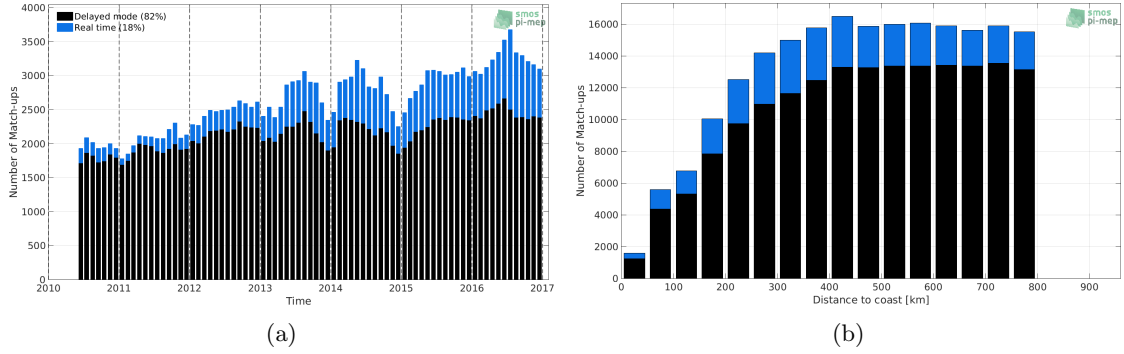
Figure 1: Number of match-ups between Argo and SMOS-L3-ICDC-V3-MONTHLY-0.5DEG SSS as a function of time (a) and as function of the distance to coast (b) over the SMOS coastal zone (<800km) 60N-60S Pi-MEP region and for the full satellite product period.
