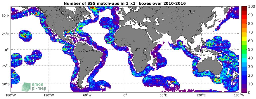
Figure 4: Number of SSS match-ups between Argo SSS and the SMOS-L3-ICDC-V3-MONTHLY-0.5DEG SSS product for the SMOS coastal zone (<800km) 60N-60S Pi-MEP region over 1°x1° boxes and for the full satellite product period.
