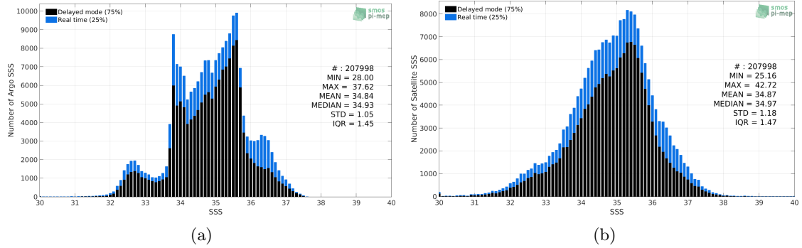
Figure 2: Histograms of SSS from Argo (a) and SMOS-L3-ICDC-V3-MONTHLY-0.5DEG (b) considering all match-up pairs per bins of 0.1 over the SMOS coastal zone ( \pm 800\text{km} ) 60N-60S Pi-MEP region and for the full satellite product period.
