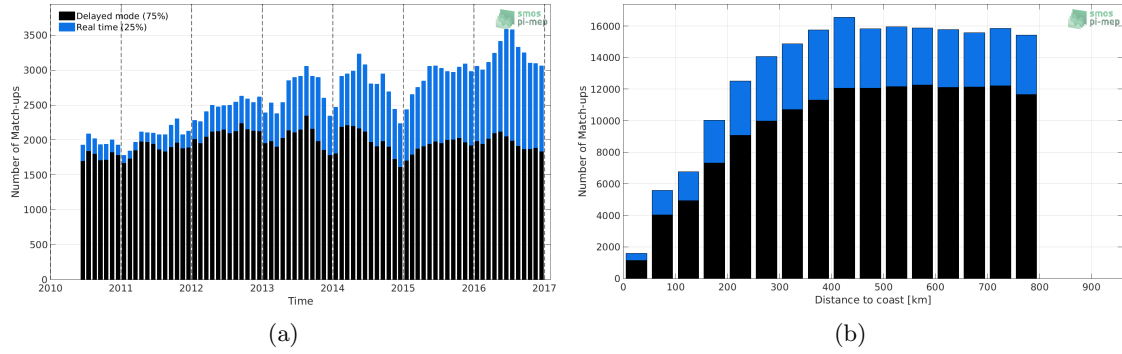
Figure 1: Number of match-ups between Argo and SMOS-L3-ICDC-V3-MONTHLY-0.5DEG SSS as a function of time (a) and as function of the distance to coast (b) over the SMOS coastal zone ( \pm 800 km) 60N-60S Pi-MEP region and for the full satellite product period.
