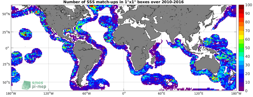
Figure 4: Number of SSS match-ups between Argo SSS and the SMOS-L3-ICDC-V3-MONTHLY-0.5DEG SSS product for the SMOS coastal zone ( \leq 800\text{km} ) 60N-60S Pi-MEP region over 1^\circ \times 1^\circ boxes and for the full satellite product period.
