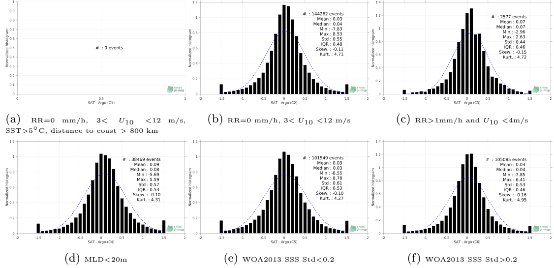
Figure 13: Normalized histogram of \Delta\text{SSS} (SMOS-L3-ICDC-V3-MONTHLY-0.5DEG - Argo) for 6 different subdatasets corresponding to: RR=0 mm/h, 3 < U_{10} < 12 m/s, SST > 5^\circ\text{C} , distance to coast > 800 km (a), RR=0 mm/h, 3 < U_{10} < 12 m/s (b), RR > 1\text{mm/h} and U_{10} < 4\text{m/s} (c), MLD < 20\text{m} (d), WOA2013 SSS Std < 0.2 (e), WOA2013 SSS Std > 0.2 (f).
