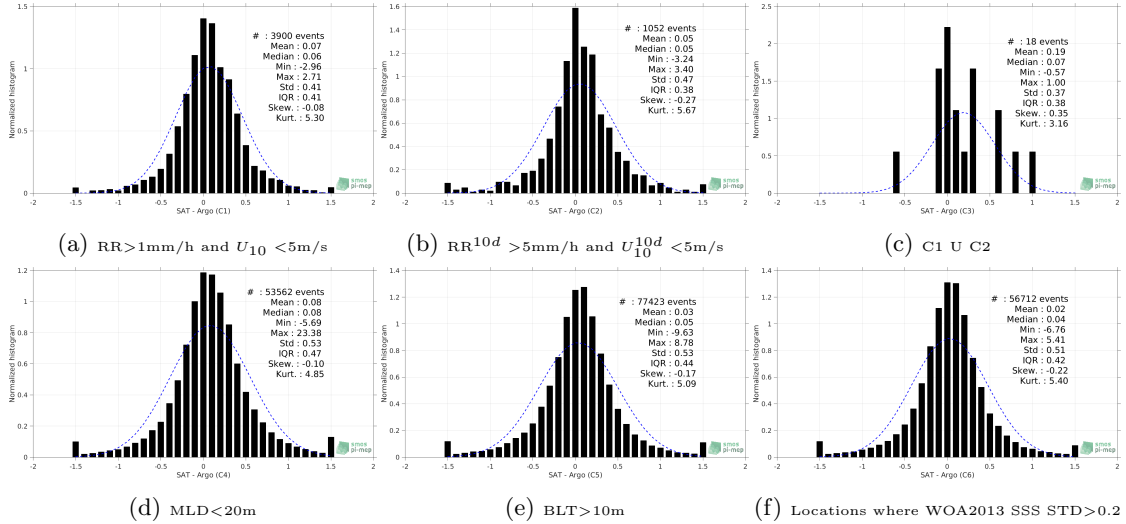
Figure 13: Normalized histogram of \Delta\text{SSS} (SMOS-L3-ICDC-V3-MONTHLY-0.5DEG - Argo) for 6 different subdatasets corresponding to: \text{RR} > 1\text{mm/h} and U_{10} < 5\text{m/s} (a), \text{RR}^{10d} > 5\text{mm/h} and U_{10}^{10d} < 5\text{m/s} (b), C1 U C2 (c), \text{MLD} < 20\text{m} (d), \text{BLT} > 10\text{m} (e), Locations where WOA2013 SSS STD > 0.2 (f).
