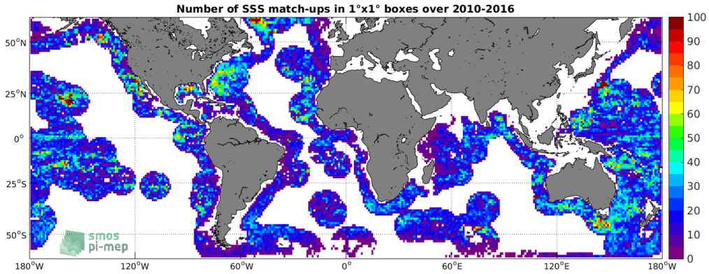
Figure 4: Number of SSS match-ups between Argo SSS and the SMOS-L3-ICDC-V3-MONTHLY-0.5DEG SSS product for the SMOS coastal zone ( \geq 800\text{km} ) 60N-60S Pi-MEP region over 1^\circ \times 1^\circ boxes and for the full satellite product period.
