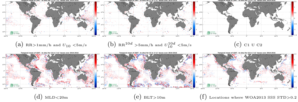
Figure 12: Temporal mean gridded over spatial boxes of size 1^\circ \times 1^\circ of \Delta\text{SSS} (SMOS-L3-ICDC-V3-MONTHLY-0.5DEG - Argo) for 6 different subdatasets corresponding to: \text{RR} > 1\text{mm/h} and U_{10} < 5\text{m/s} (a), \text{RR}^{10d} > 5\text{mm/h} and U_{10}^{10d} < 5\text{m/s} (b), C1 U C2 (c), \text{MLD} < 20\text{m} (d), \text{BLT} > 10\text{m} (e), Locations where WOA2013 SSS STD > 0.2 (f).
