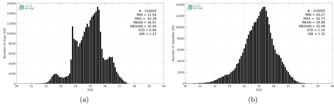
Figure 2: Histograms of SSS from Argo (a) and SMOS-L3-ICDC-V3-MONTHLY-0.5DEG (b) considering all match-up pairs per bins of 0.1 over the SMOS coastal zone ( \geq 800\text{km} ) 60N-60S Pi-MEP region and for the full satellite product period.
