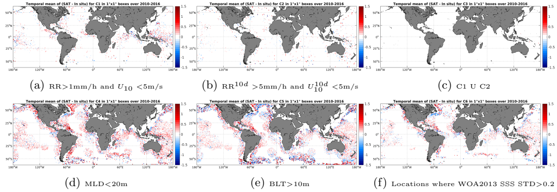
Figure 12: Temporal mean gridded over spatial boxes of size 1^\circ \times 1^\circ of \Delta SSS (SMOS-L3-ICDC-V3-MONTHLY-0.5DEG - Argo) for 6 different subdatasets corresponding to: RR > 1\text{mm/h} and U_{10} < 5\text{m/s} (a), RR^{10d} > 5\text{mm/h} and U_{10}^{10d} < 5\text{m/s} (b), C1 U C2 (c), MLD < 20\text{m} (d), BLT > 10\text{m} (e), Locations where WOA2013 SSS STD > 0.2 (f).
