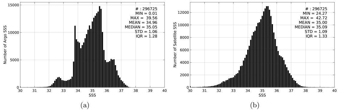
Figure 2: Histograms of SSS from Argo (a) and SMOS-L3-ICDC-V3-MONTHLY-0.5DEG (b) considering all match-up pairs per bins of 0.1 over the SMOS coastal zone ( \geq 800\text{km} ) 60N-60S Pi-MEP region and for the full satellite product period.
