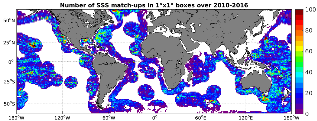
Figure 4: Number of SSS match-ups between Argo SSS and the SMOS-L3-ICDC-V3-MONTHLY-0.5DEG SSS product for the SMOS coastal zone ( \pm 800\text{km} ) 60N-60S Pi-MEP region over 1^\circ \times 1^\circ boxes and for the full satellite product period.
